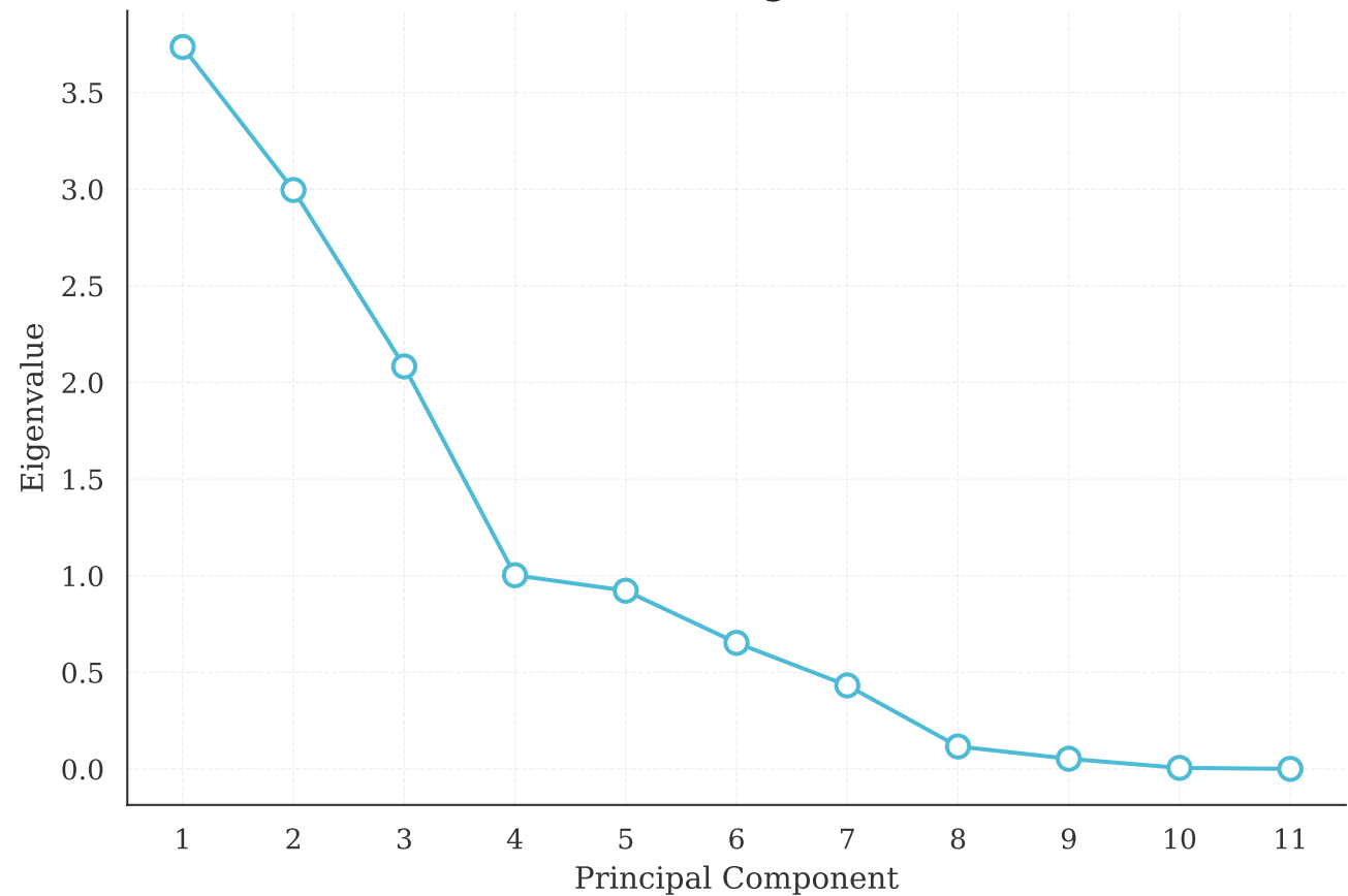
Scree Plot (Eigenvalues)
