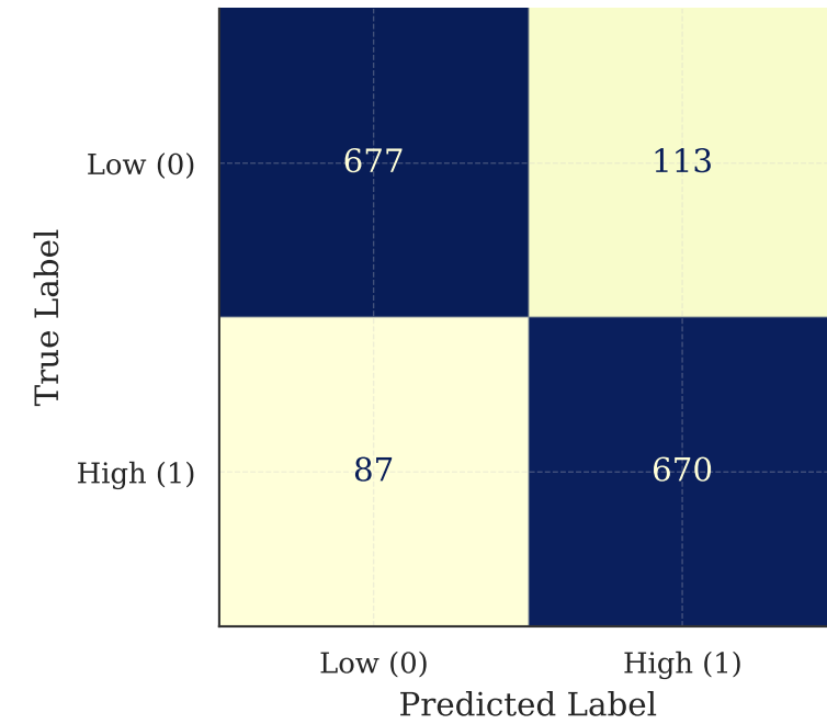
KNN (Original)
