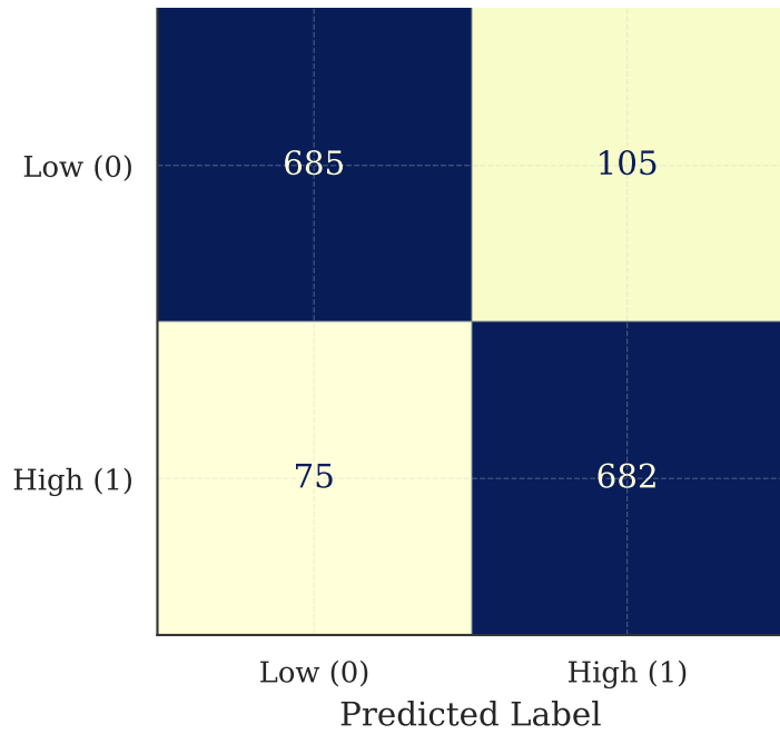
LightGBM (Original)
