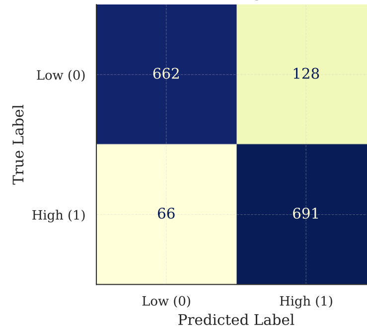
KNN (Original)
