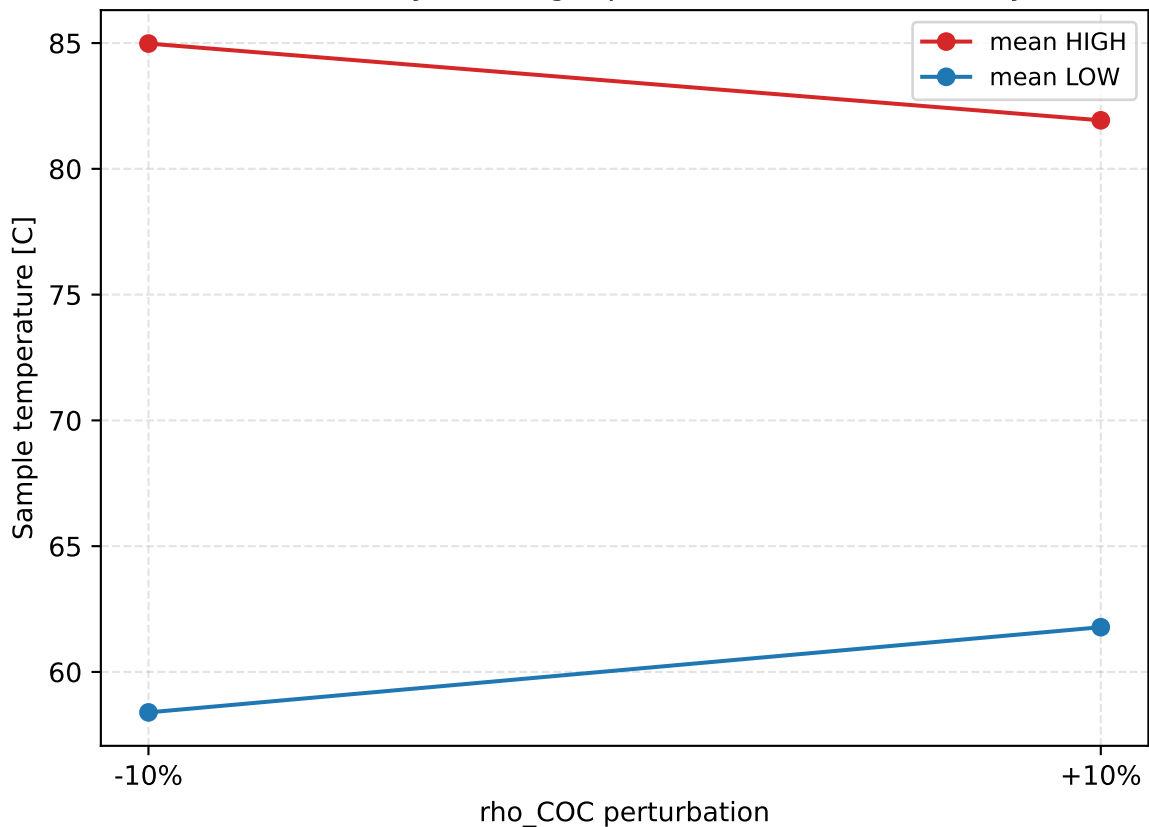
rho_COC propagation to sample prediction (identifiability warning: cp' on calibration boundary)
