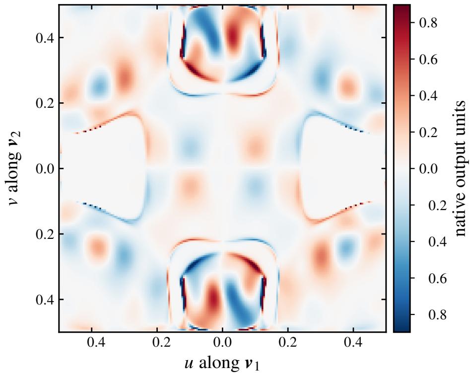
Hermitian Curvature Tensor
