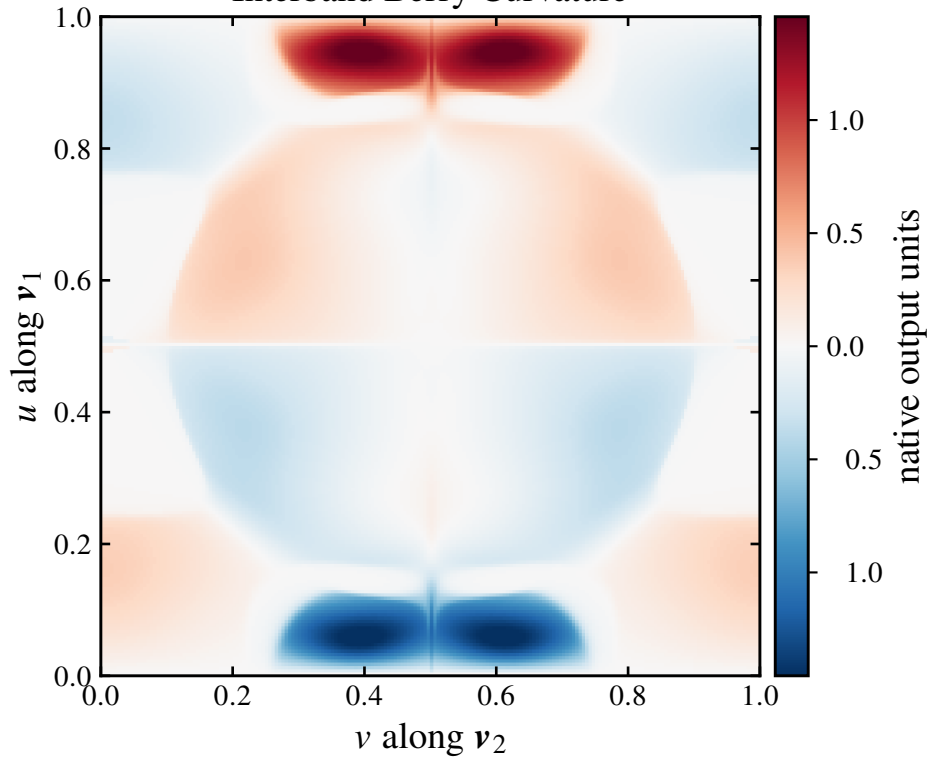
Interband Berry Curvature
