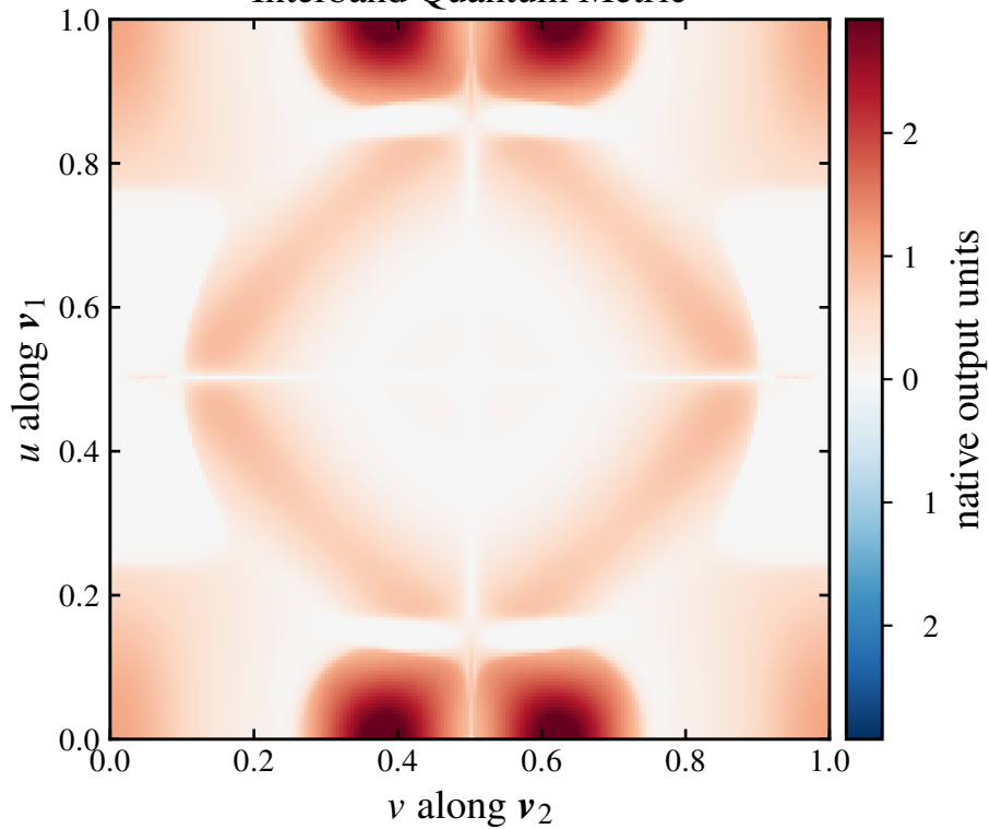
Interband Quantum Metric
