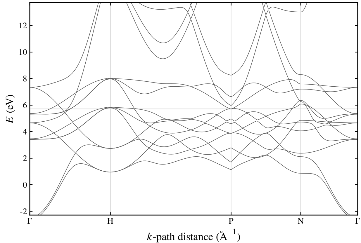
Fe SOC first-principles bands
