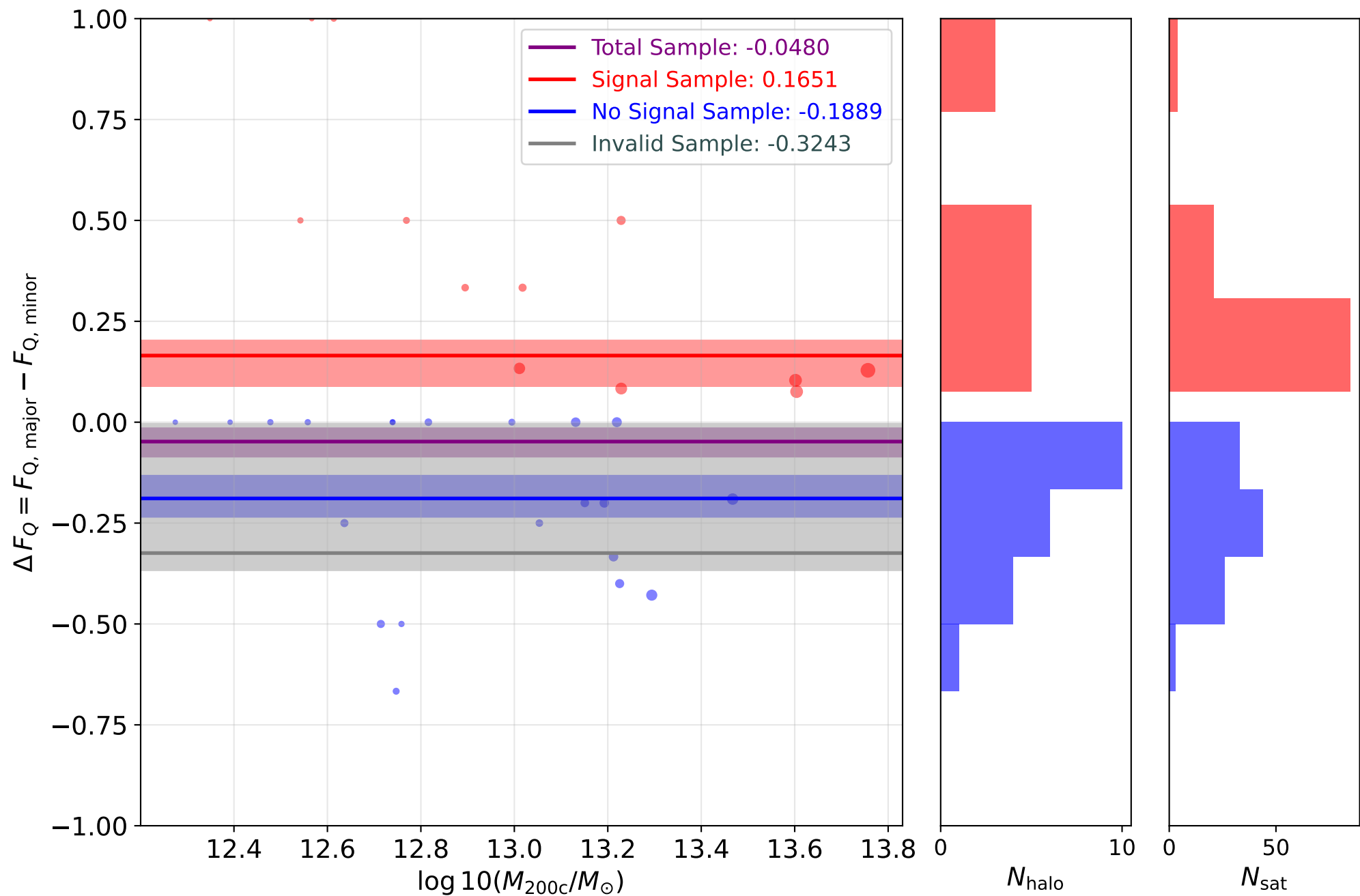
EAGLE: ASGQ Signal per Cluster halo-axis. z=0.0
