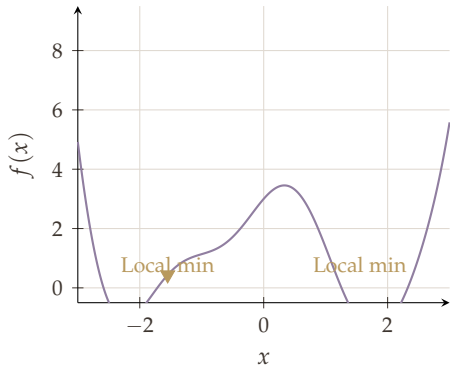
Non-Convex
