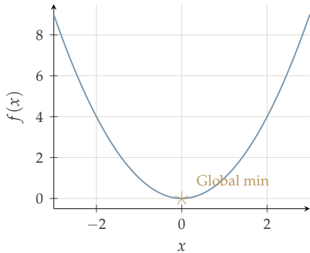
Convex
