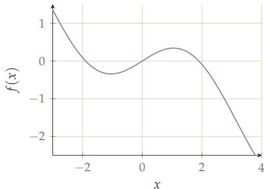
Unbounded ( f^* = -\infty )
