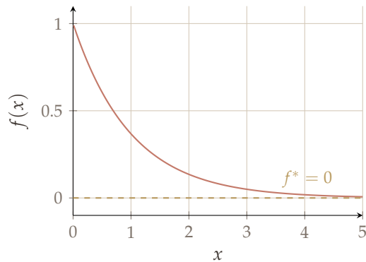
f^* = 0 , x^* does not exist
