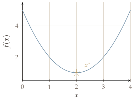
Unique x^*
