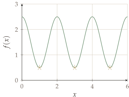
Non-unique x^*
