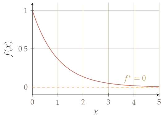
f^* = 0 , x^* does not exist
