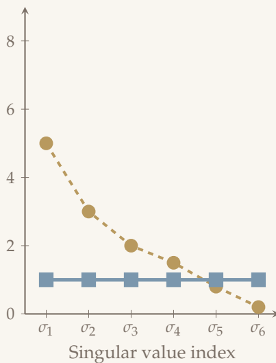
Mid Training
