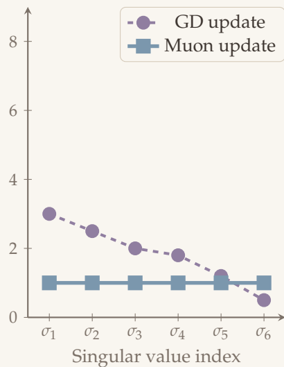
Late Training
