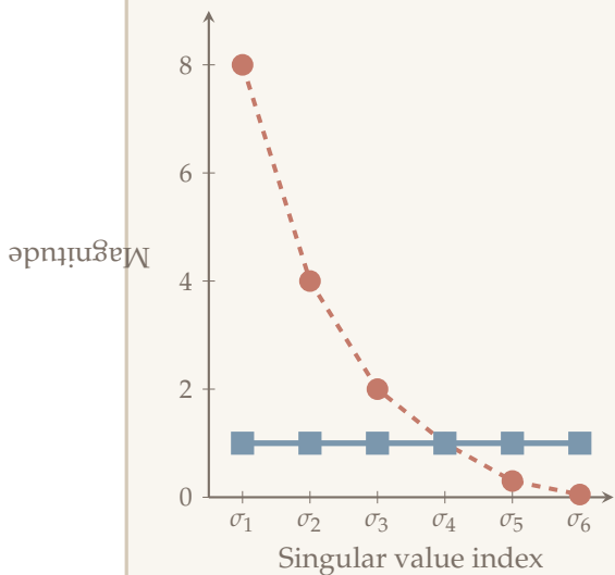
Early Training
