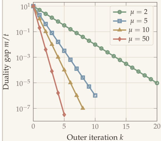
Duality gap vs. outer iteration
