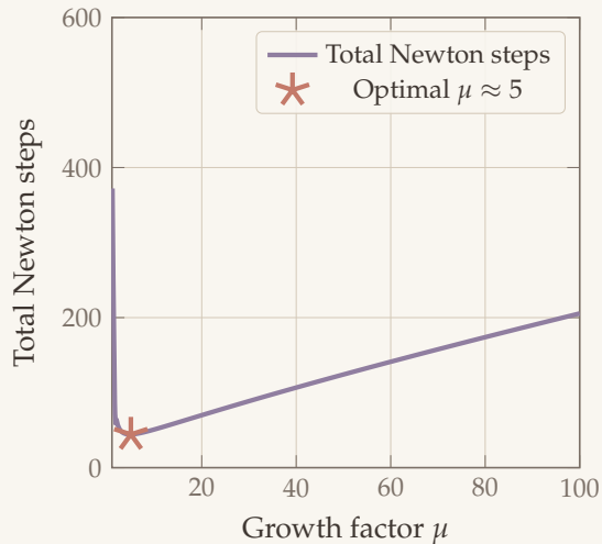
Total Newton steps vs. \mu
