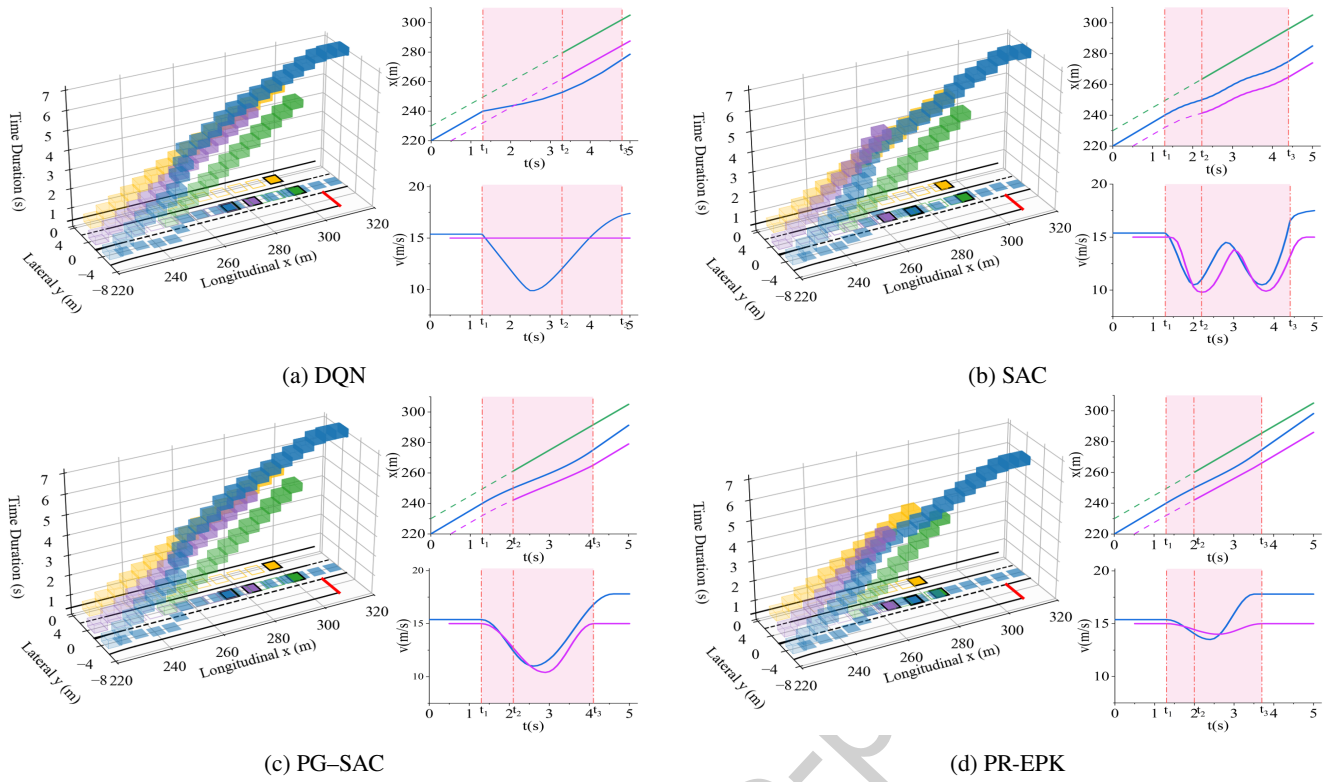
Figure 6: Spatiotemporal visualization of EV merging in dynamic traffic: the 3D diagram shows EV/SVs occupancy in longitudinal-lateral-time space, and the right panels show the corresponding x-t and v-t profiles. In the x-t plot, green/magenta/blue denote the lead vehicle, lag vehicle, and EV trajectories, respectively. t_1 , t_2 , and t_3 mark lane-change initiation, entry into the target lane, and merge completion. (a) DQN. (b) SAC. (c) PG-SAC. (d) PR-EPK.
