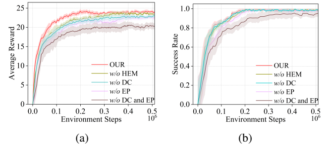
Figure 8: The training results of ablation study, (a) the average reward of different ablation method in training process, (b) the success rate of different ablation method in training process.
