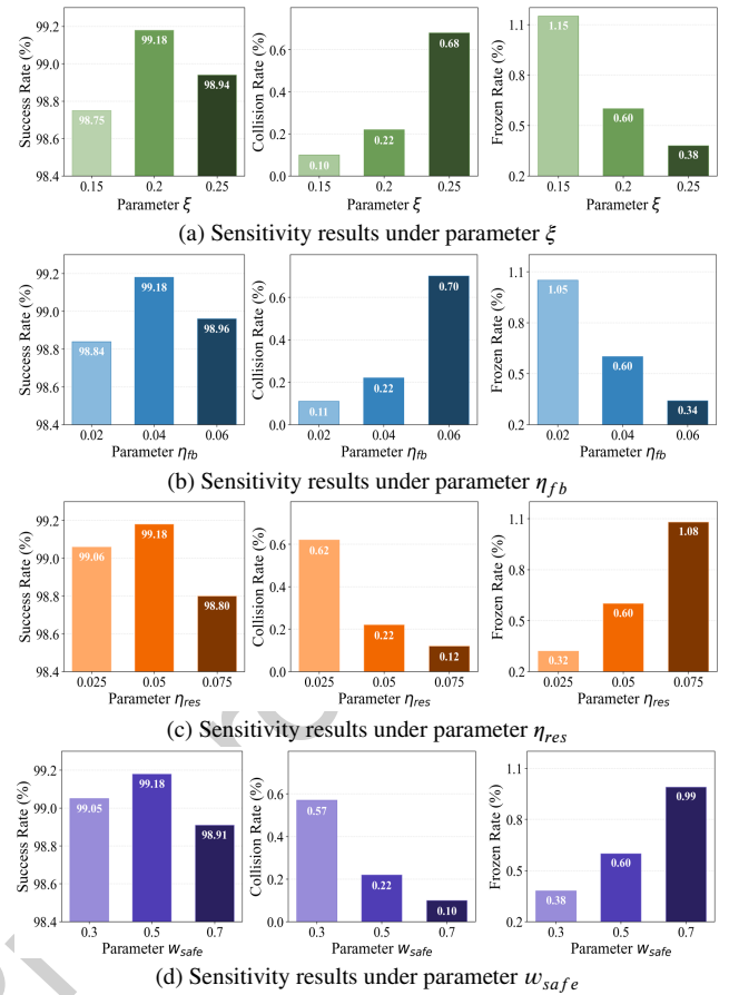
Figure 7: Parameter sensitivity analysis. Rows represent parameters \xi , \eta_{fb} , \eta_{res} , and w_{safe} ; columns display success, collision, and frozen rates.
