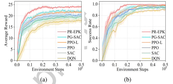
Figure 4: (a) The average reward of different RL agent in training process. (b) The success rate of different RL agent in training process.
