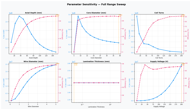
Figure 11. Parameter sensitivity sweeps around the optimised baseline (NdFeB N52, L = 150 mm, d_{\text{core}} = 39 mm, N = 200 , d_w = 5 mm, \delta = 0.05 mm, V = 200 V). Blue: P_{\text{fan}} ; pink dashed: \eta ; orange vertical line: baseline value.
