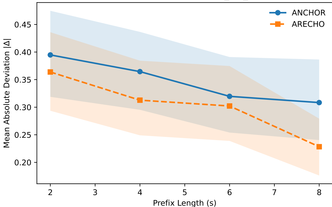
Robustness Curve — nisqa_noi_pred
