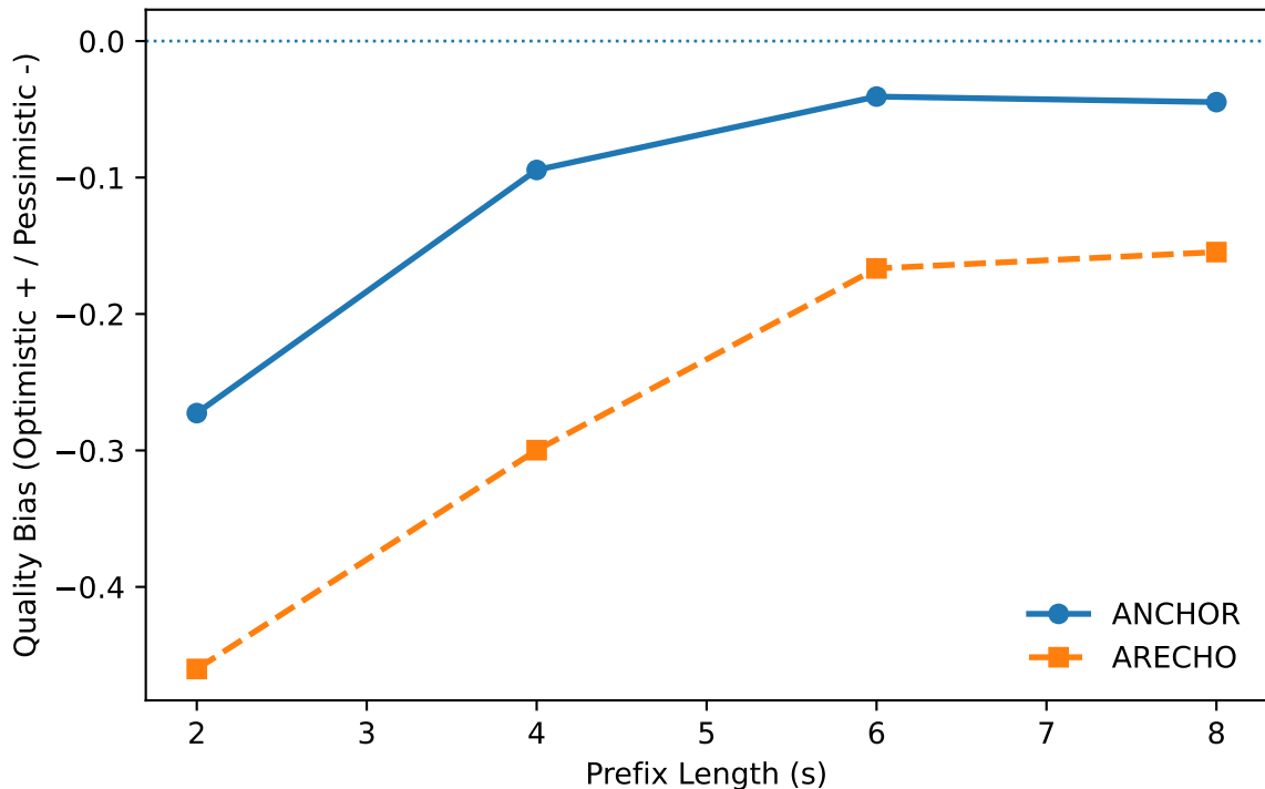
Directional Quality Bias — utmosv2 ↑ (Higher Better)
