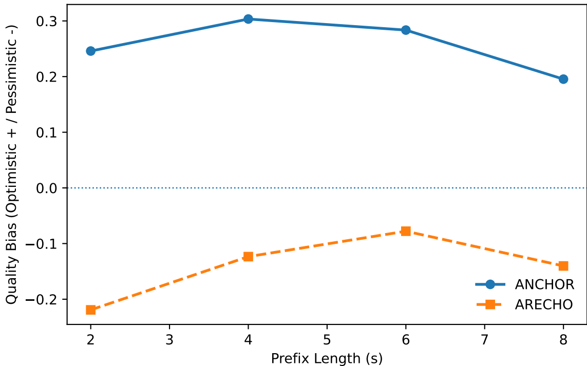
Directional Quality Bias — plcmos ↑ (Higher Better)
