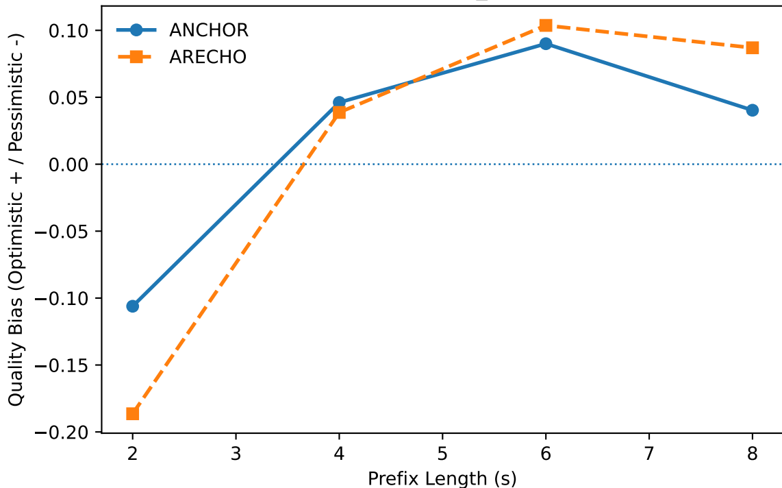
Directional Quality Bias — dns_p808 ↑ (Higher Better)
