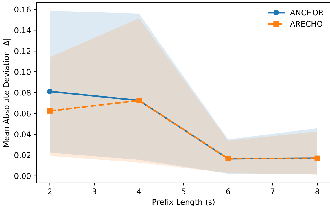
Robustness Curve — asr_match_error_rate
