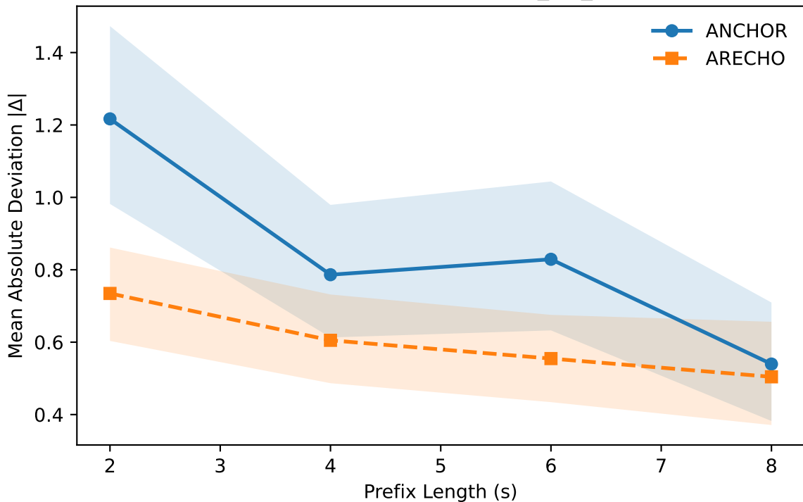
Robustness Curve — nisqa_dis_pred
