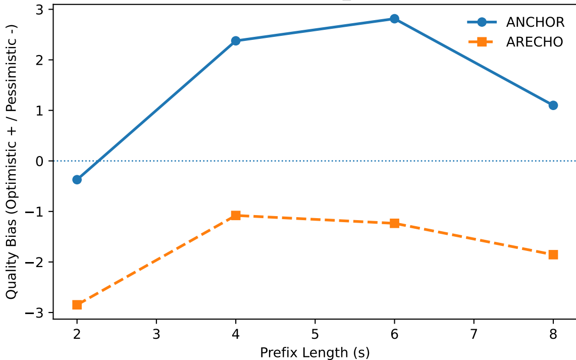
Directional Quality Bias — se_sdr \uparrow (Higher Better)
