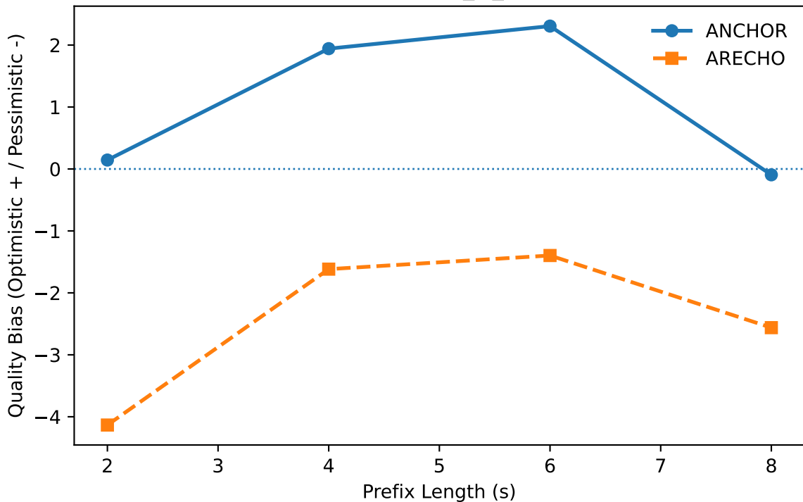
Directional Quality Bias — se_si_snr \uparrow (Higher Better)
