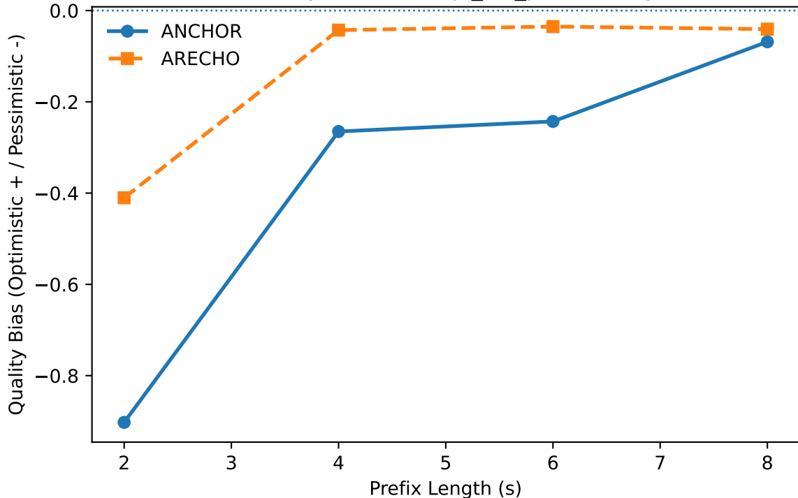
Directional Quality Bias — nisqa_dis_pred ↑ (Higher Better)
