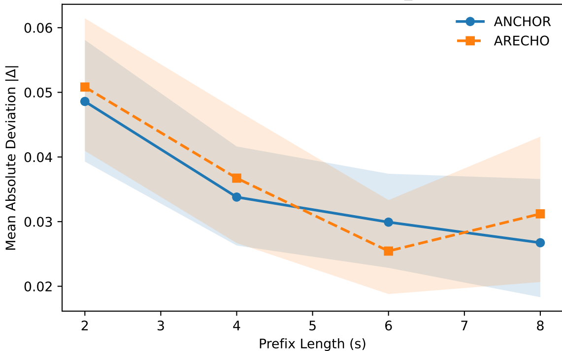
Robustness Curve — speech_bert
