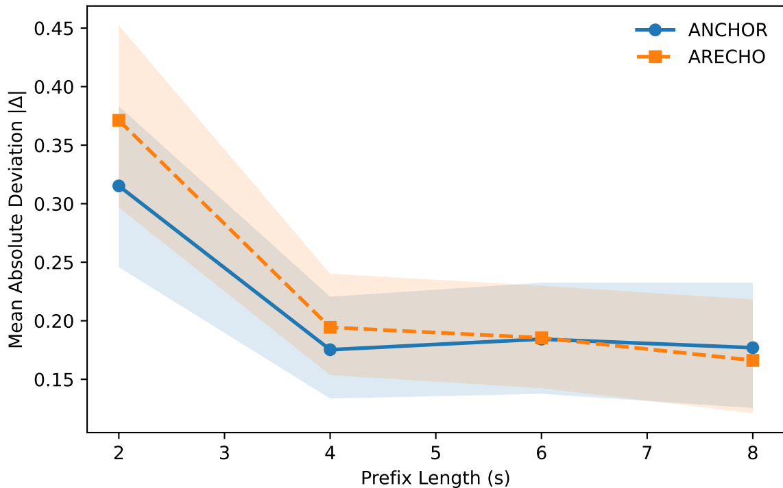
Robustness Curve — utmos
