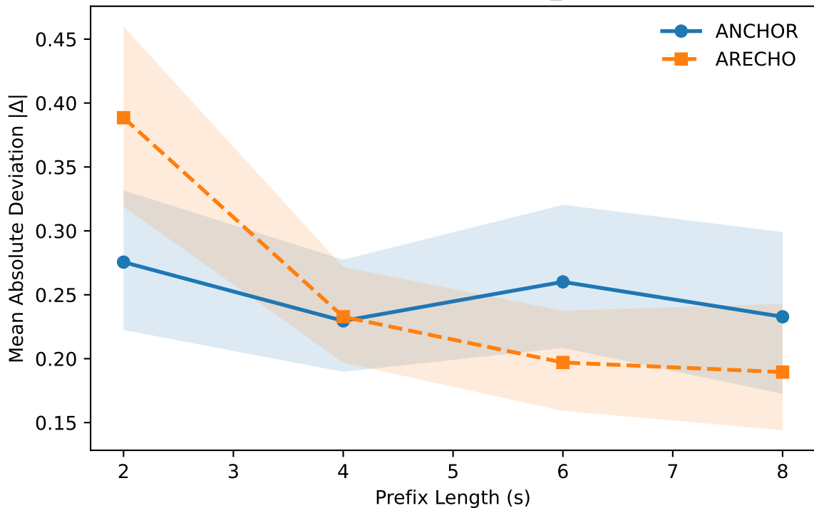
Robustness Curve — dns_overall
