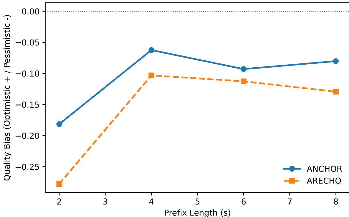
Directional Quality Bias — utmos ↑ (Higher Better)
