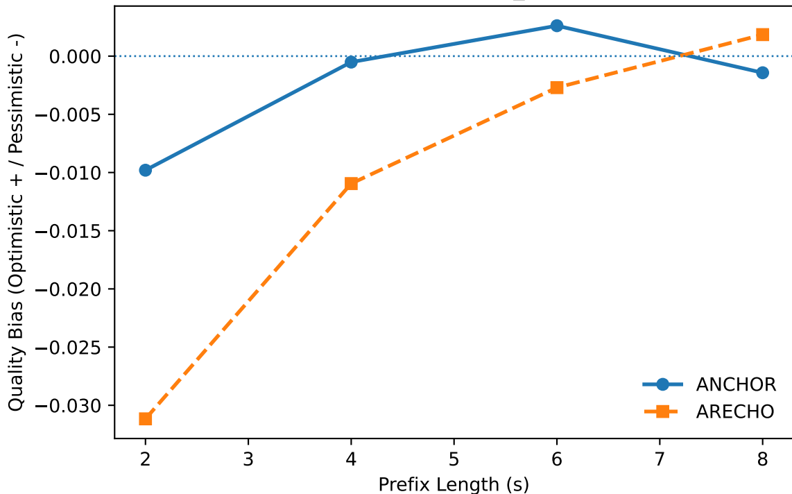
Directional Quality Bias — speech_bert ↑ (Higher Better)
