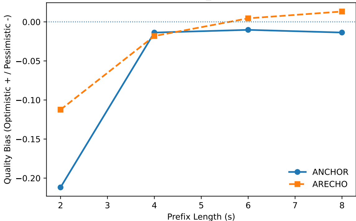
Directional Quality Bias — spk_similarity ↑ (Higher Better)
