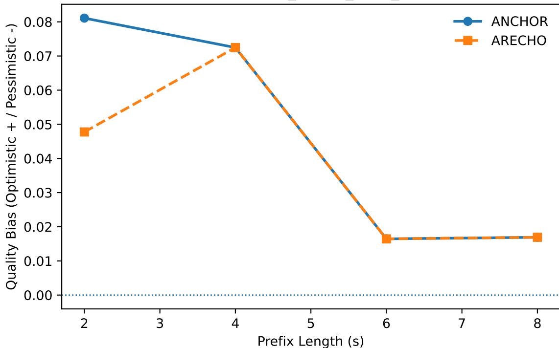
Directional Quality Bias — asr_match_error_rate ↓ (Lower Better)
