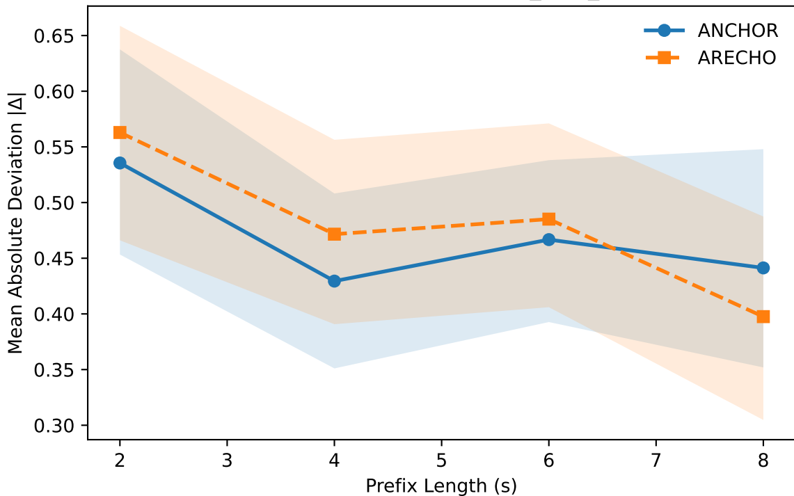
Robustness Curve — nlsqa_mos_pred
