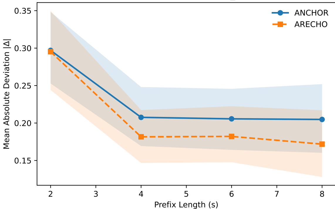
Robustness Curve — dns_p808
