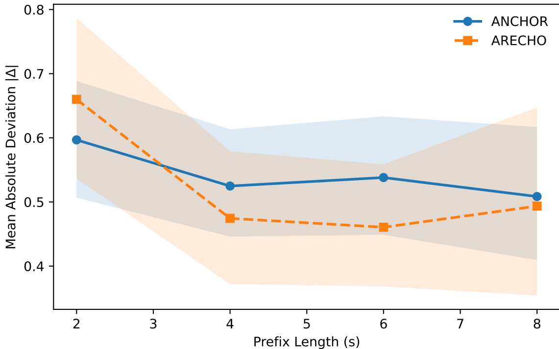
Robustness Curve — plcmos
