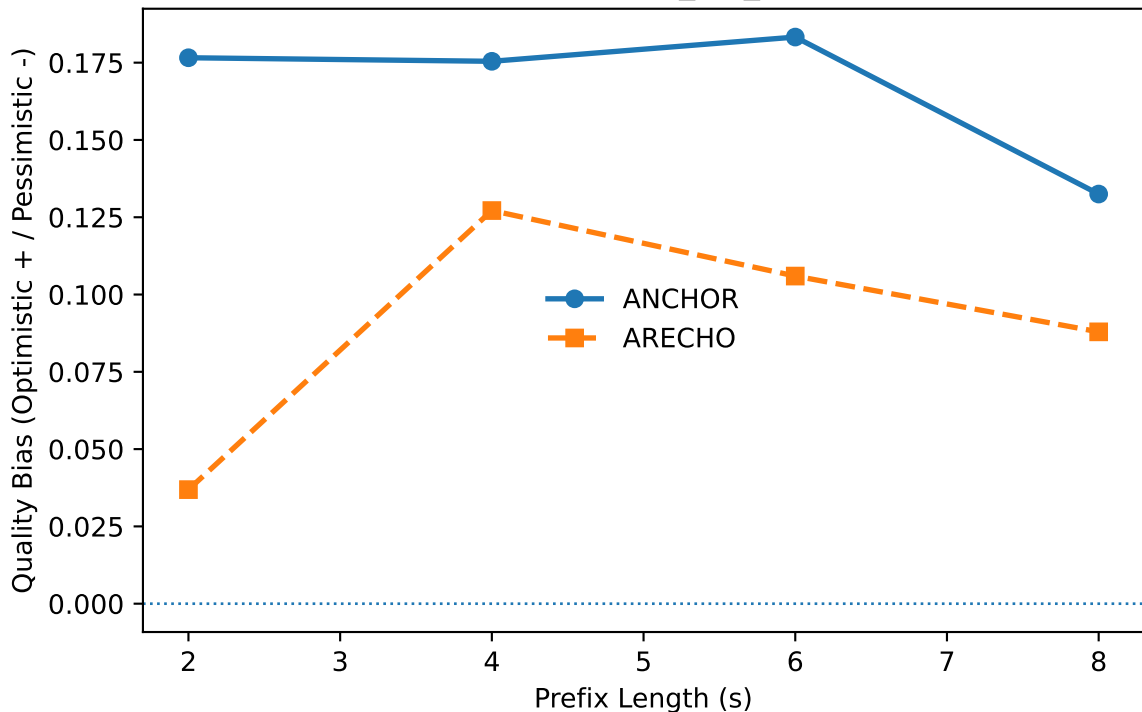
Directional Quality Bias — nisqa_noi_pred ↑ (Higher Better)
