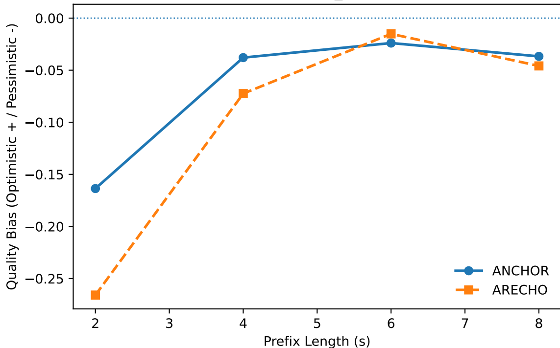
Directional Quality Bias — dns_overall \uparrow (Higher Better)
