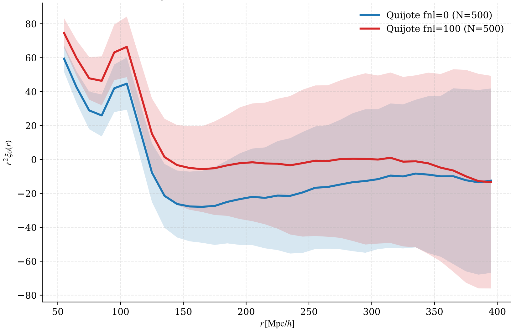
Quijote Measured 2PCF Mean: fnl=0 vs fnl=100
