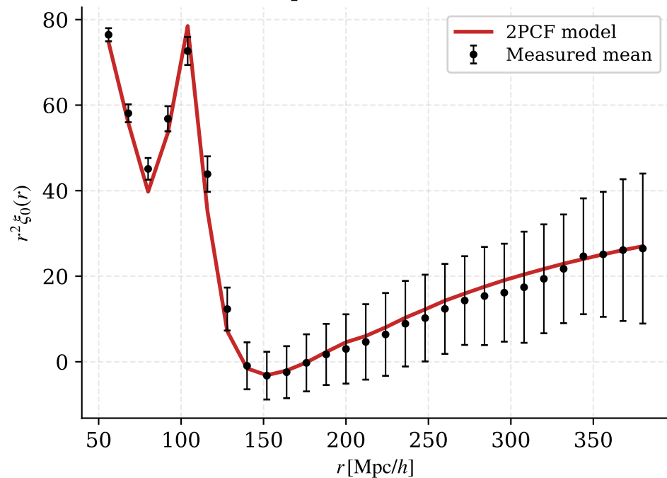
3Gpc fastPM fnl100
