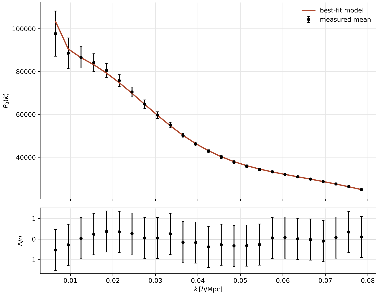
Task50 rawbox_commonkmin1000_shot_sigmas0 P(k) fit
