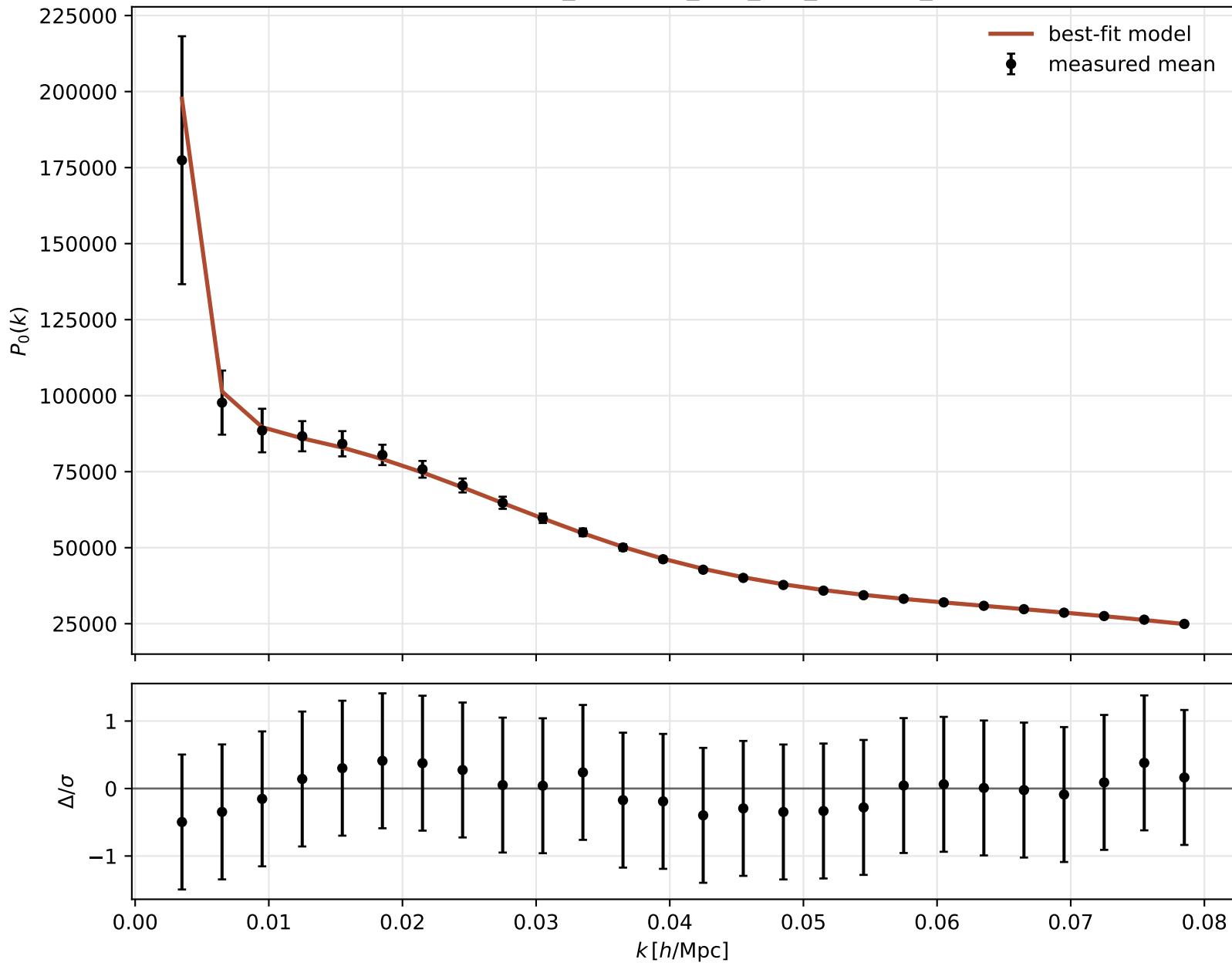
Task4.2 P(k) rawbox_ownkmin_free_sn0_sigmas0_z1 P(k) fit
