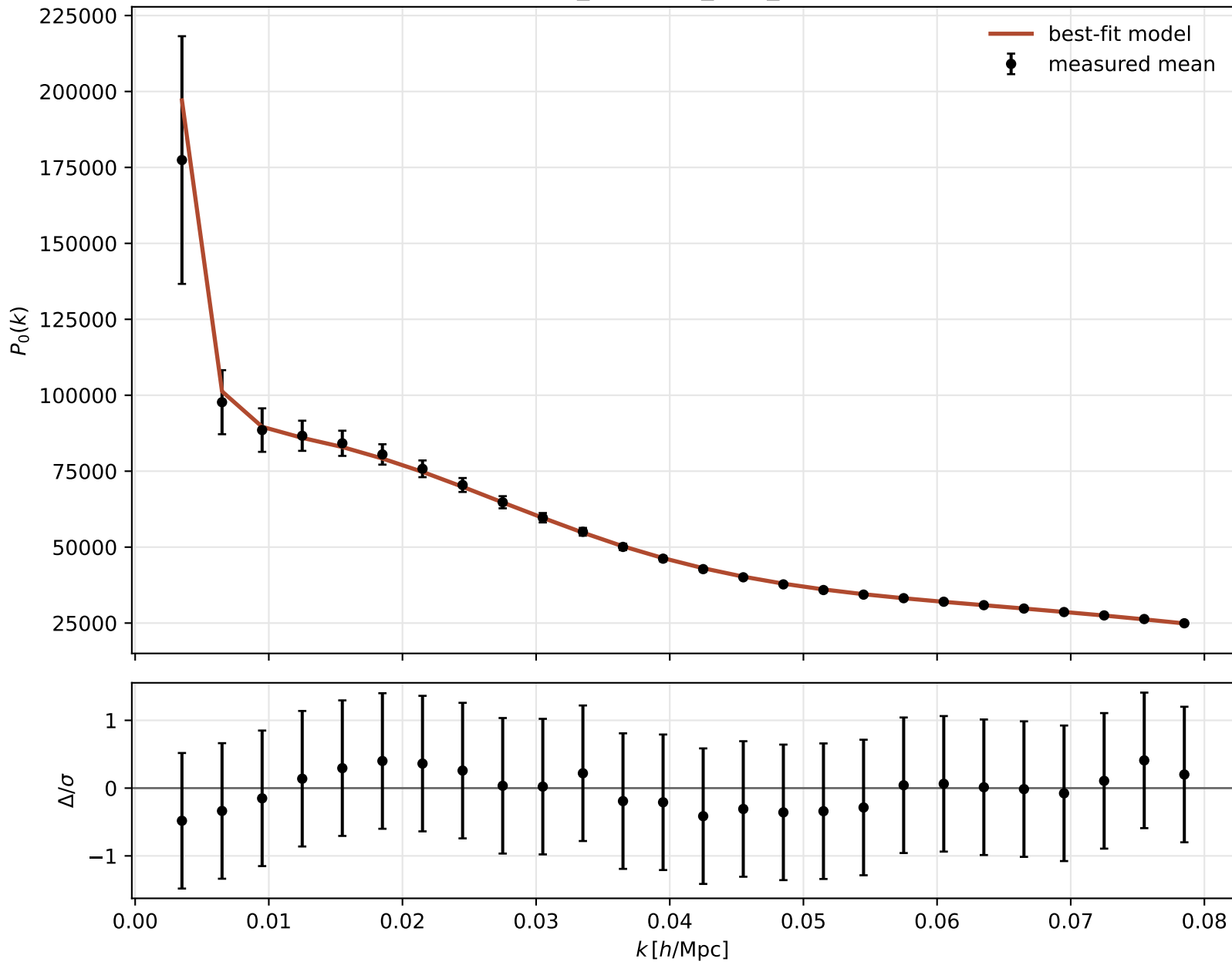
Task50 rawbox_ownkmin_shot_sigmas0 P(k) fit
