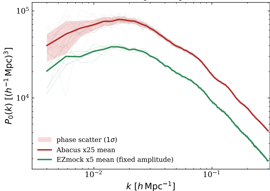
Periodic-box power spectrum
