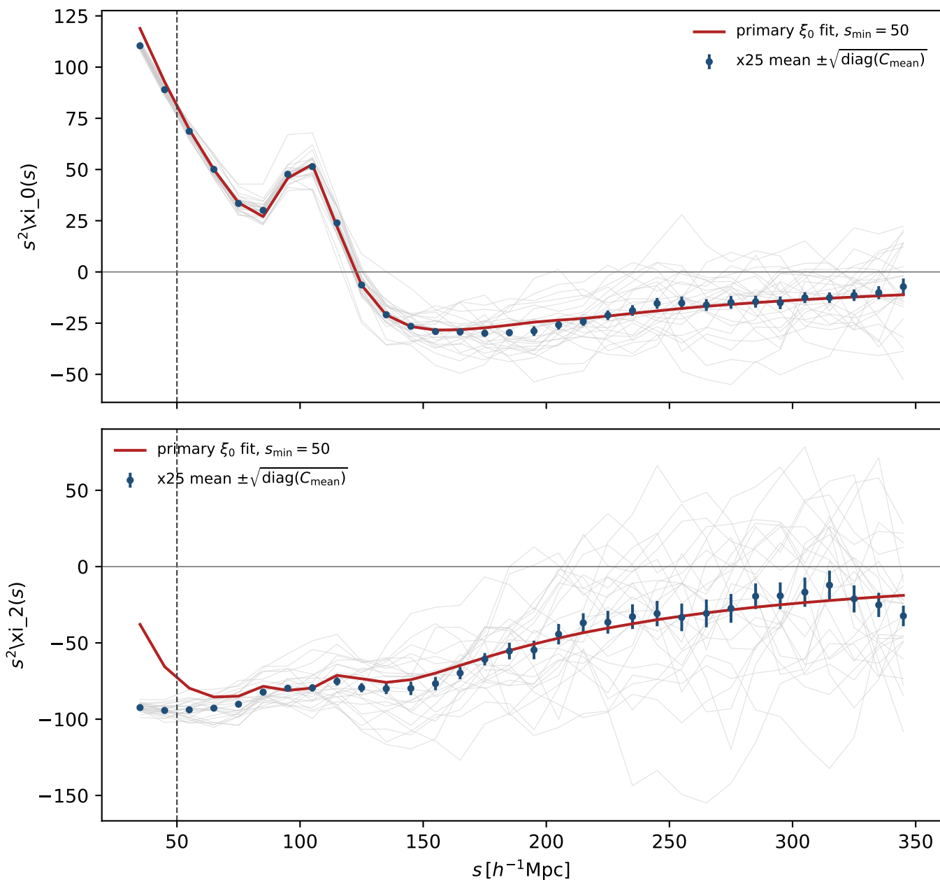
Task 4.3.2 rawbox x25: f_{\text{NL}} = -1.07 \pm 6.97 (single-volume convention)
