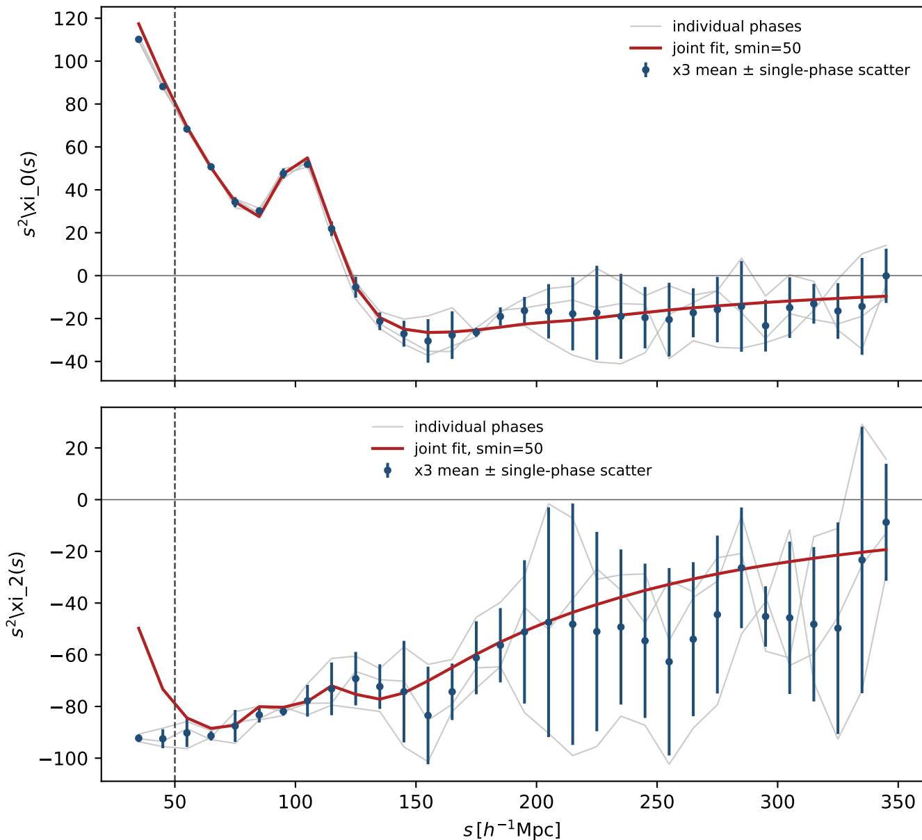
Task 4.3.2 rawbox x3 pilot: f_{\text{NL}} = 5.7 , b_1 = 2.590 , \sigma_s = 6.74
