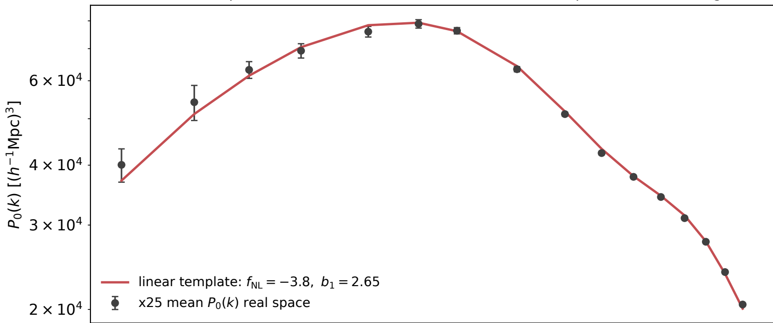
rawbox real space P0, frozen 16 bins ( k=0.003..0.095 ), exact parent-mode average
