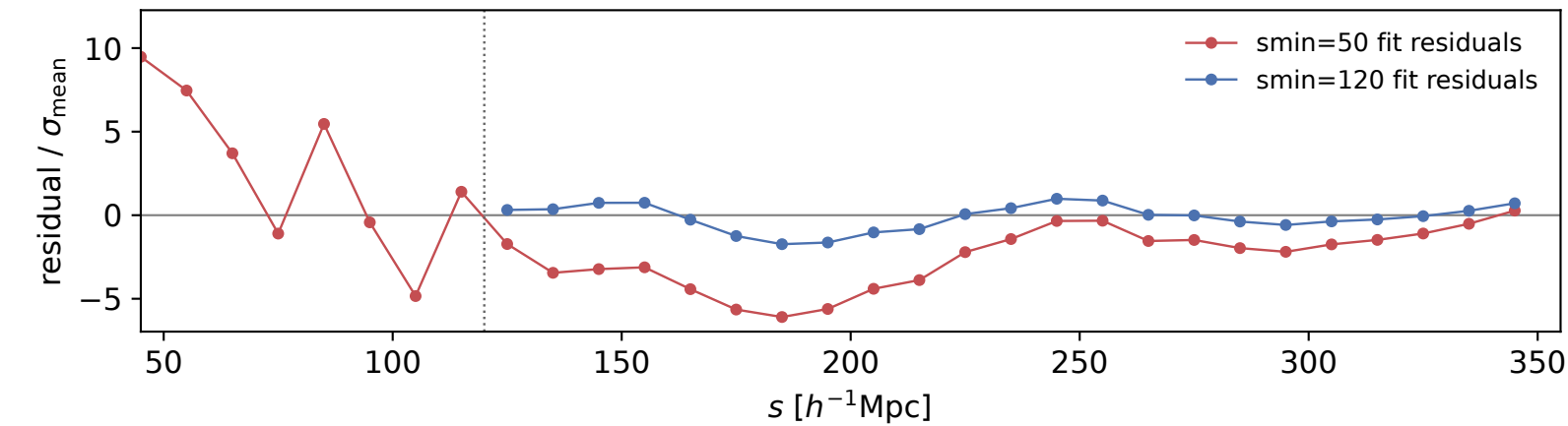
smin=50: \chi^2 = 331/28 , PTE = 1.3 \times 10^{-121} ; smin=120: \chi^2 = 24.1/21 , PTE = 0.29
