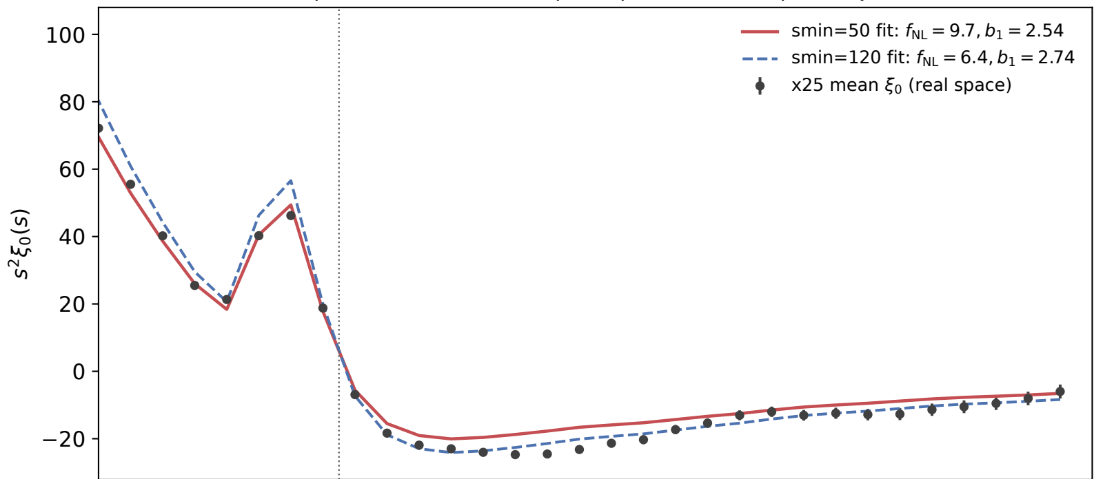
rawbox real space, no FoG / Kaiser / quadrupole: linear template + j0 shell kernels
