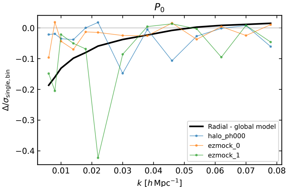
Measured shuffled - reference changes: one halo and two EZ mocks Qualitative check only; C_single is not the paired covariance
