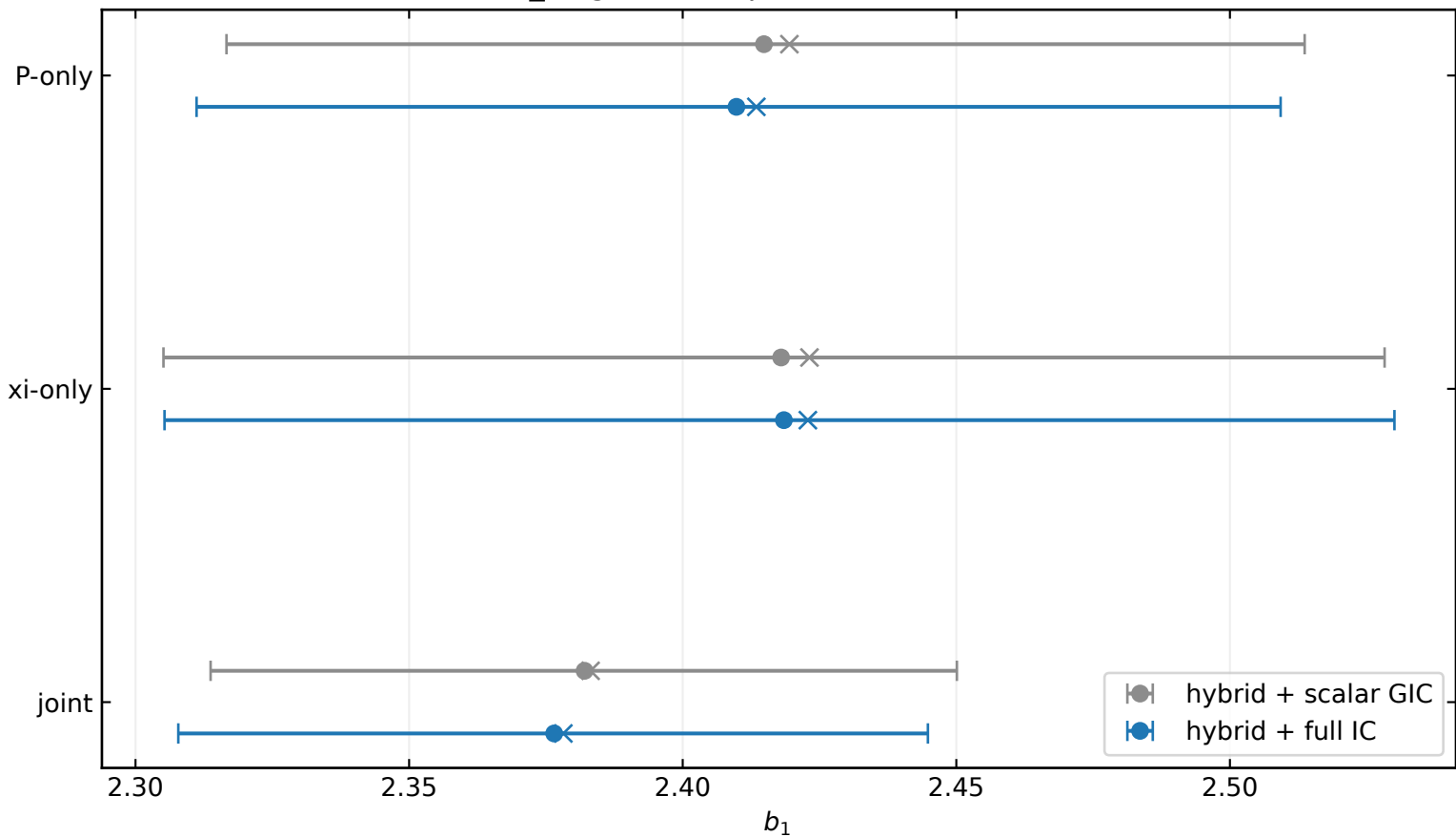
Bias constraints: median with 68% interval; crosses mark MAP EZmock1000 C_single, Hartlap likelihood and Percival intervals
