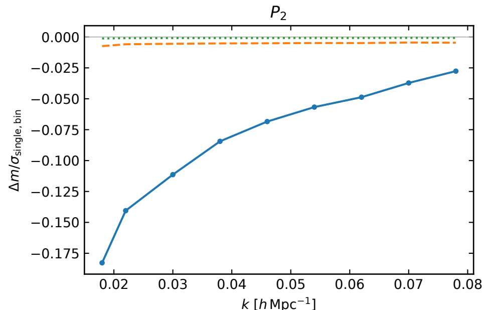
Deterministic model changes at the full-IC joint MAP Same parameters, frozen EZmock1000 covariance
