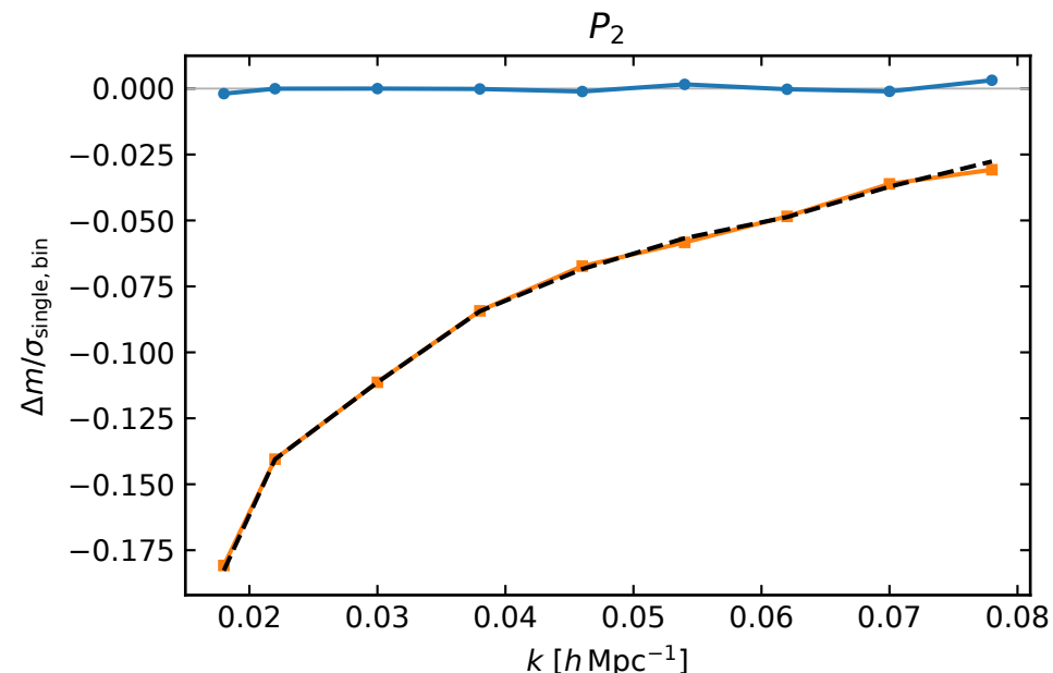
Separate global prescription changes from additional radial IC Common full-IC joint MAP; fixed Poisson and existing sn0 included
