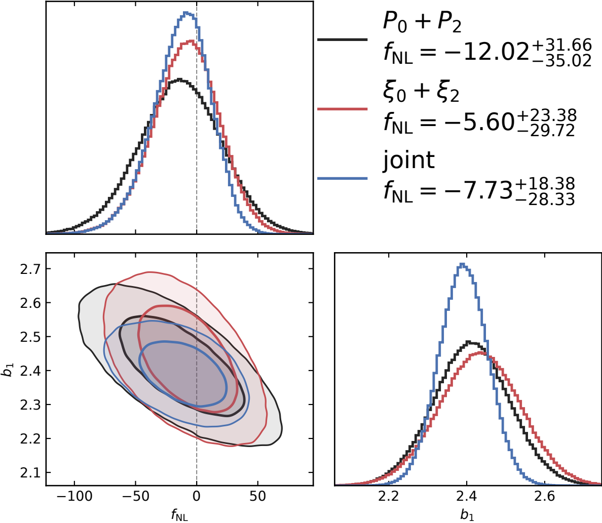
Task43 lightcone RSD (box-safe 0.4 < z_{\text{obs}} < 0.8 ; k_{\text{max}}=0.08 , s_{\text{min}}=50 ): P02, BAO-masked xi02, and joint — jaxpower analytic (hybrid xi) covariance
