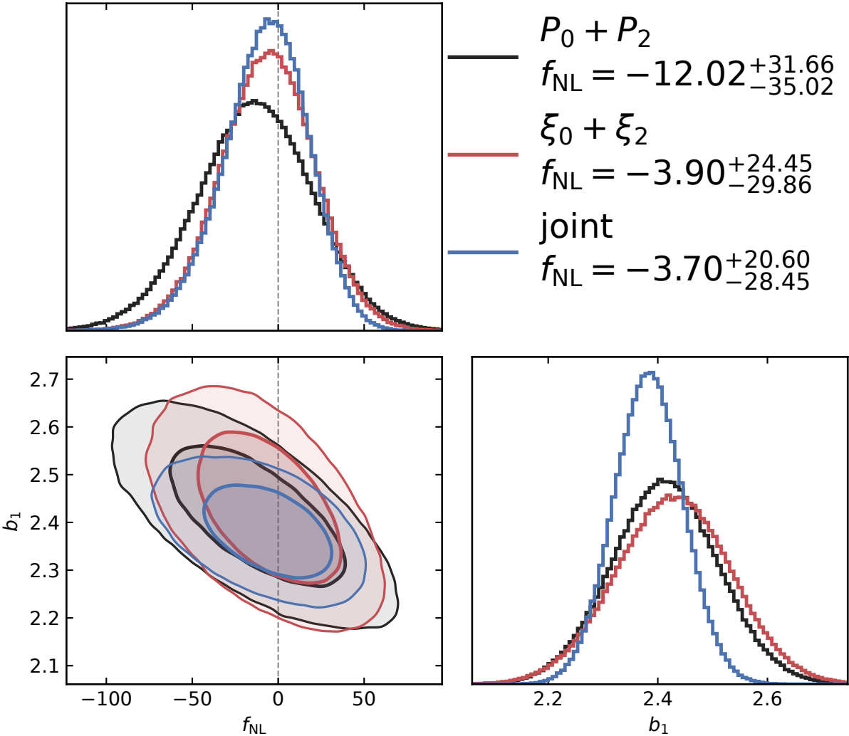
Hybrid xi + fixed-window GIC; no extra free parameter
