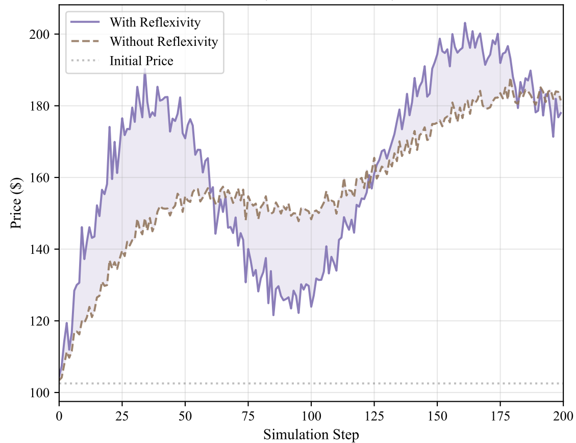
(a) Reflexivity Effect on Price Dynamics
