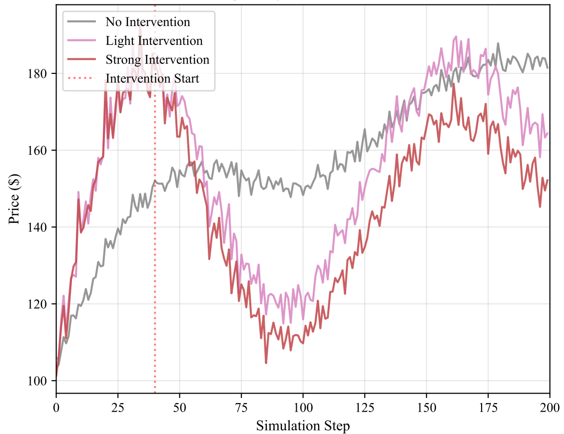
(b) Regulatory Intervention Effects
