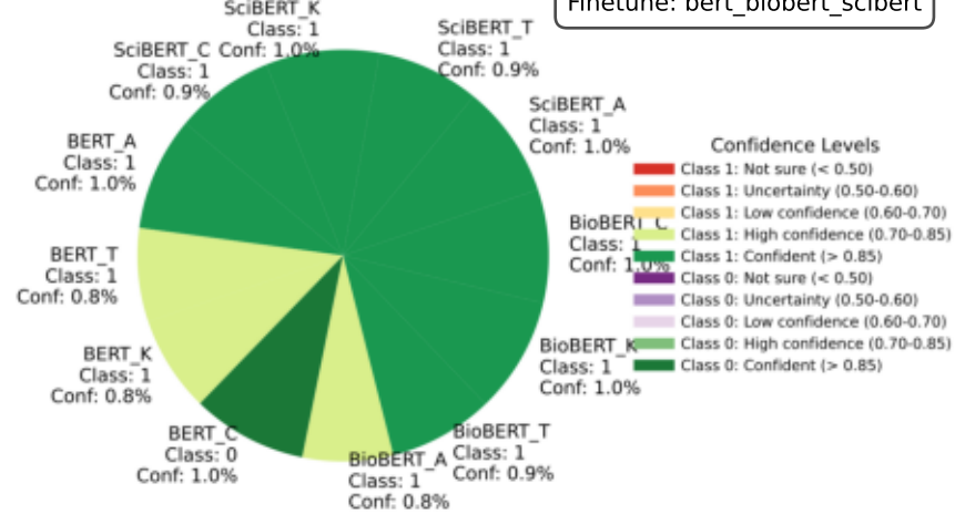
Study 9990
