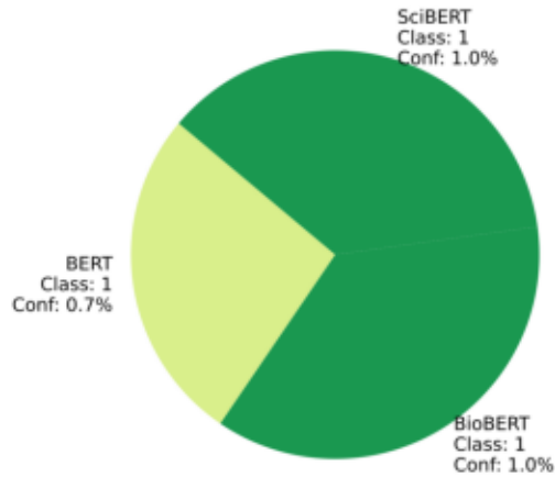
Study 9990
