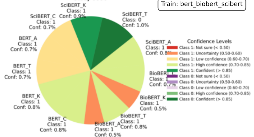
Study 9990
