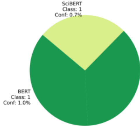
Study 9990
