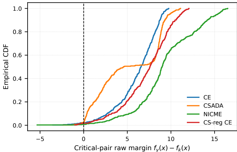
PMI-20 critical-pair margins
