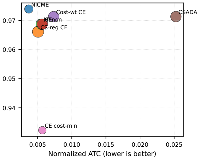
Target-macro recall
