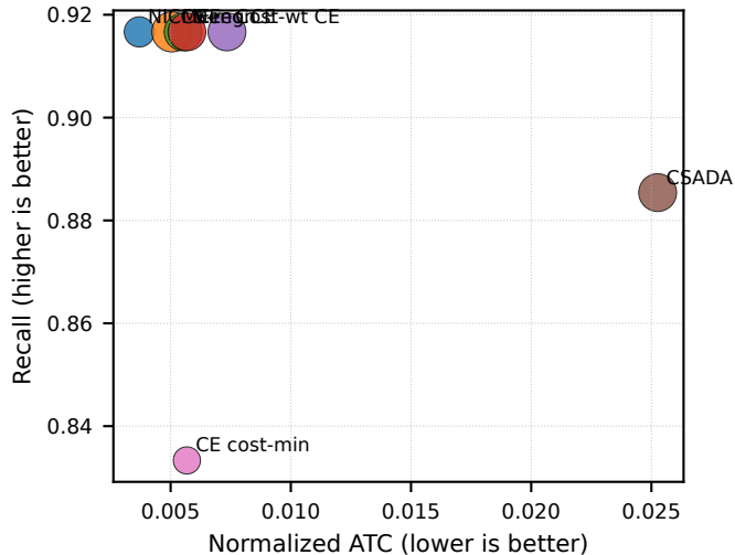
Target-min recall
