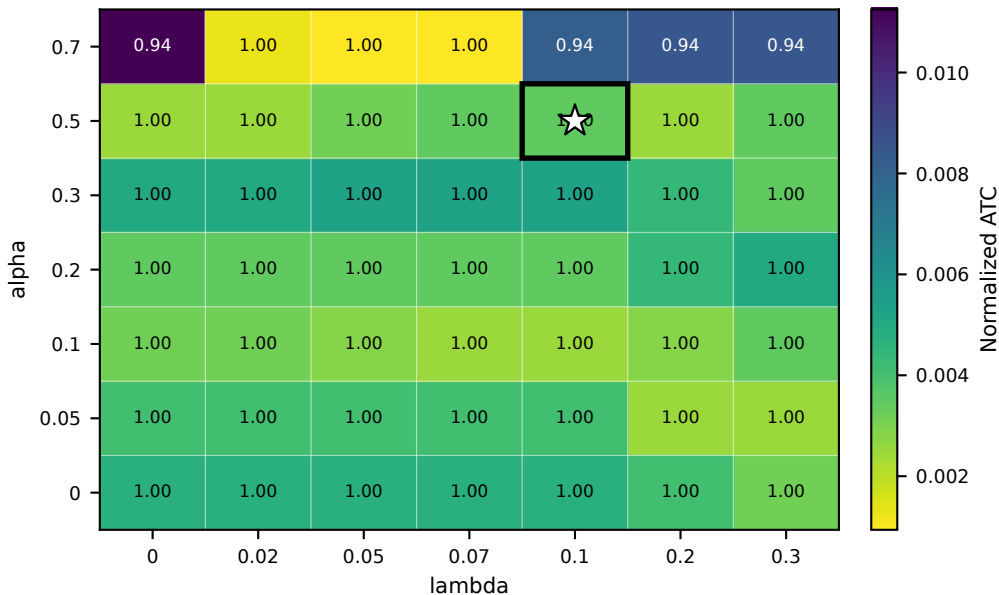
PMI-20 NICME validation heatmap
