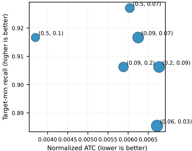
PMI-20 NICME sensitivity
