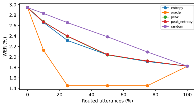
Fig. 1. Router ablation on dev-clean. Risk-aware ordering improves over random routing, while the oracle exposes remaining headroom.
