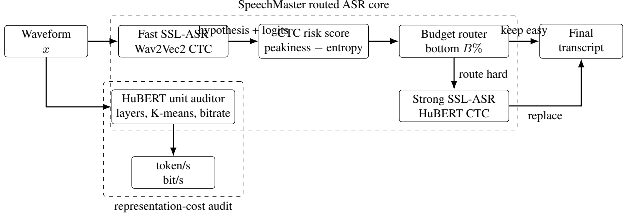
Fig. 1. Overview of SpeechMaster. The routed ASR core trades WER against RTF, while the unit auditor quantifies discrete SSL representation cost.
