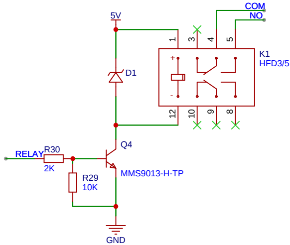
COM/NO继电器
