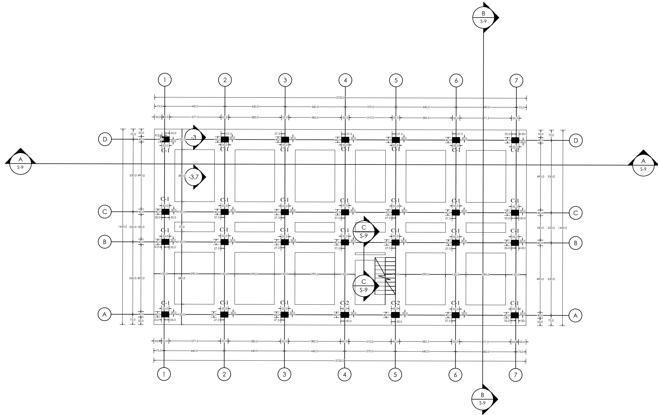
04 | REF. | SCALE: 1:100 Foundation PLAN and Column Layout
