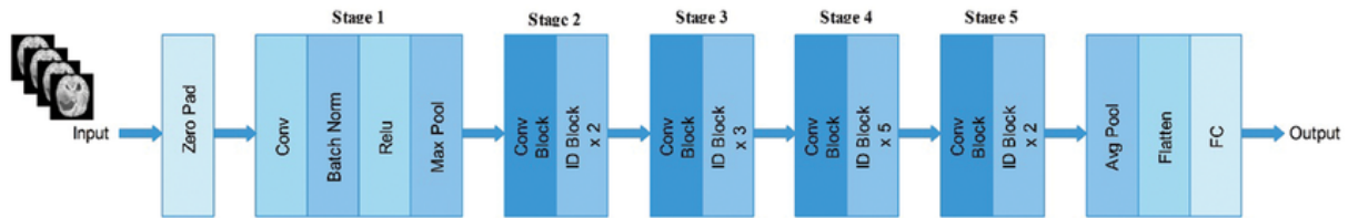
Figure 3.5: Architecture of the ResNet50 illustrating the successive stages of the model.
