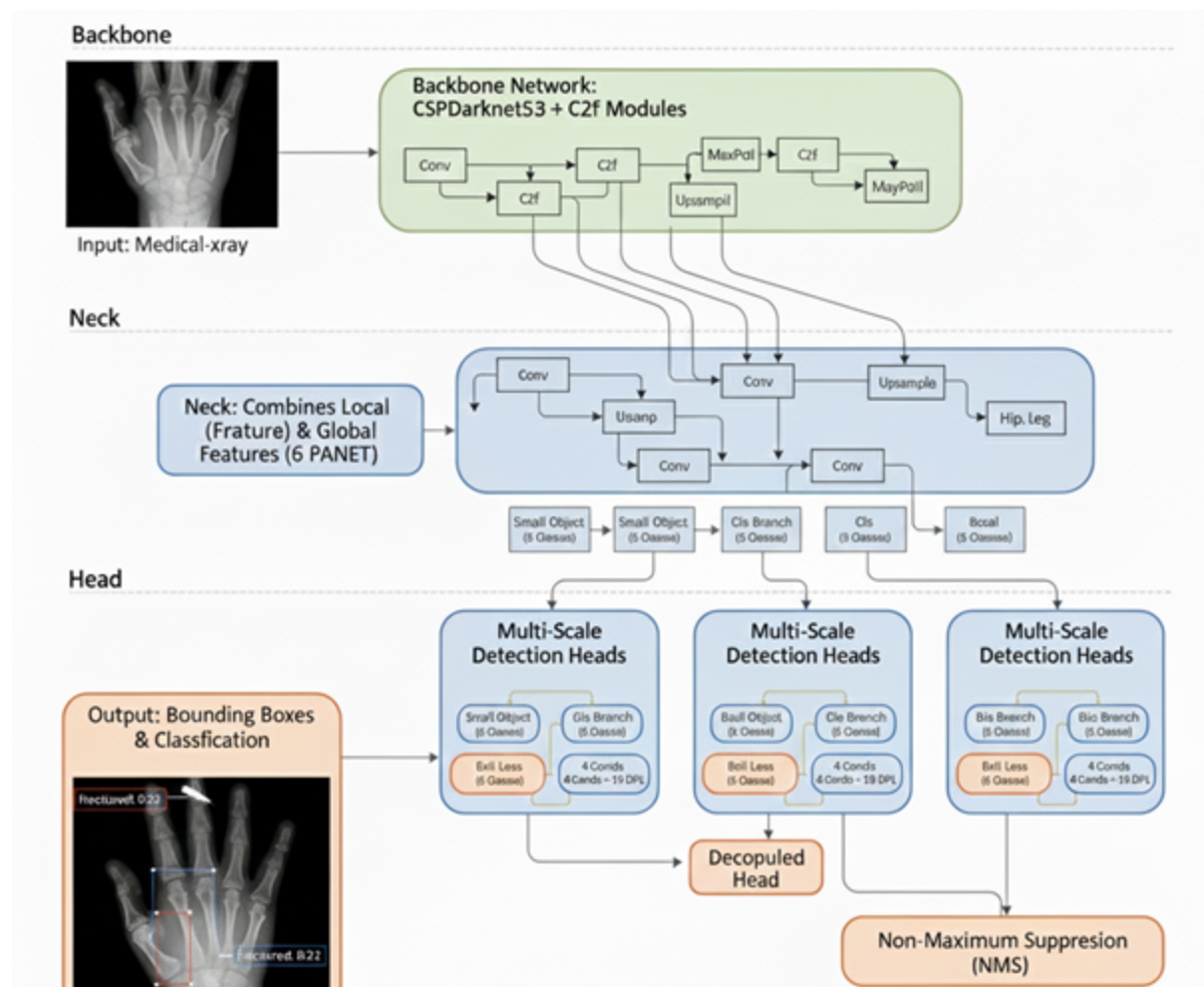
Figure 3.6: Architecture of the YOLOv8 illustrating the successive stages of the model.
