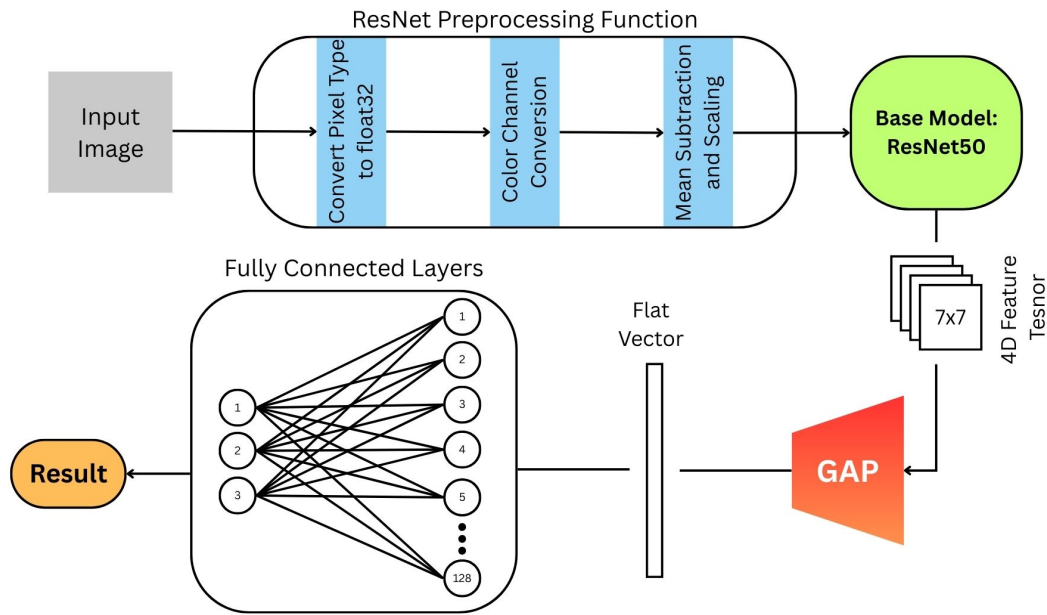
Figure 3.7: Overall architecture of the proposed medical image routing model.
