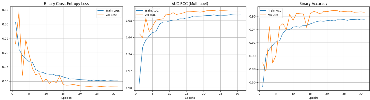
Figure 4.18: Learning curves for ResNet50 OVR.
