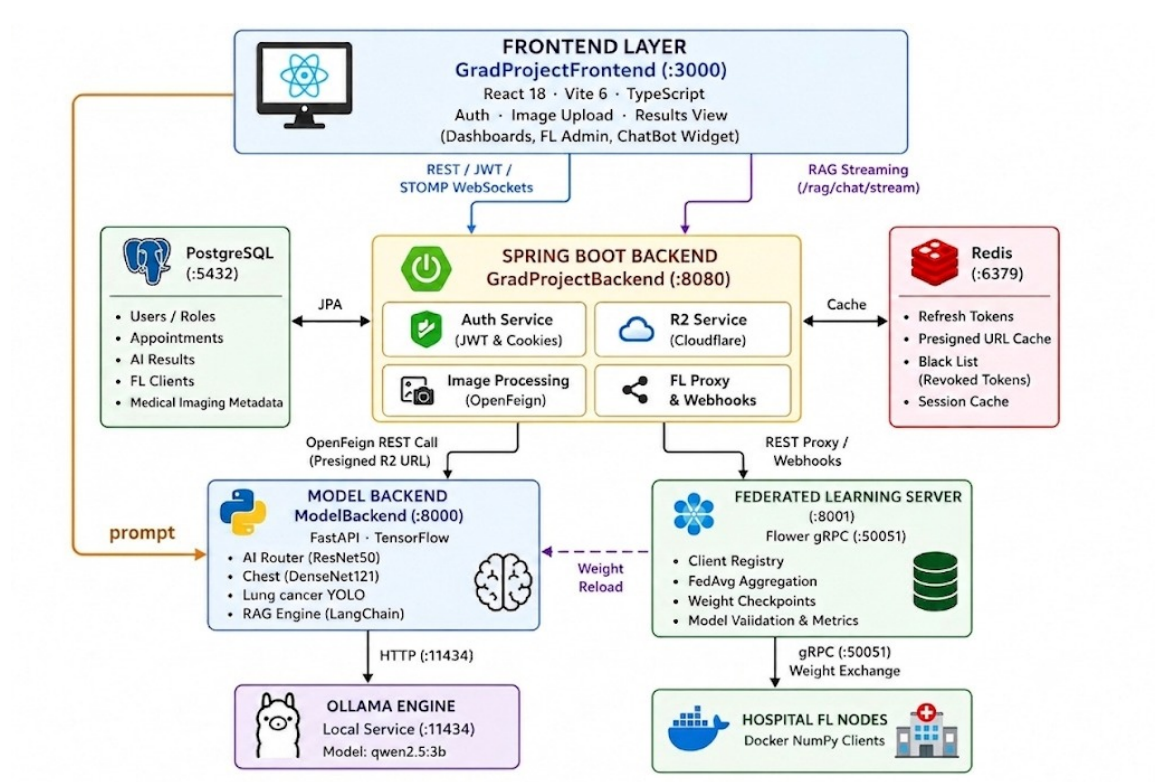
Figure 3.32: End-to-end logical architecture of the proposed X-Fed NeuroScan framework, illustrating the interaction between users, backend services, AI models, explainability components, federated learning infrastructure, and data storage systems.
