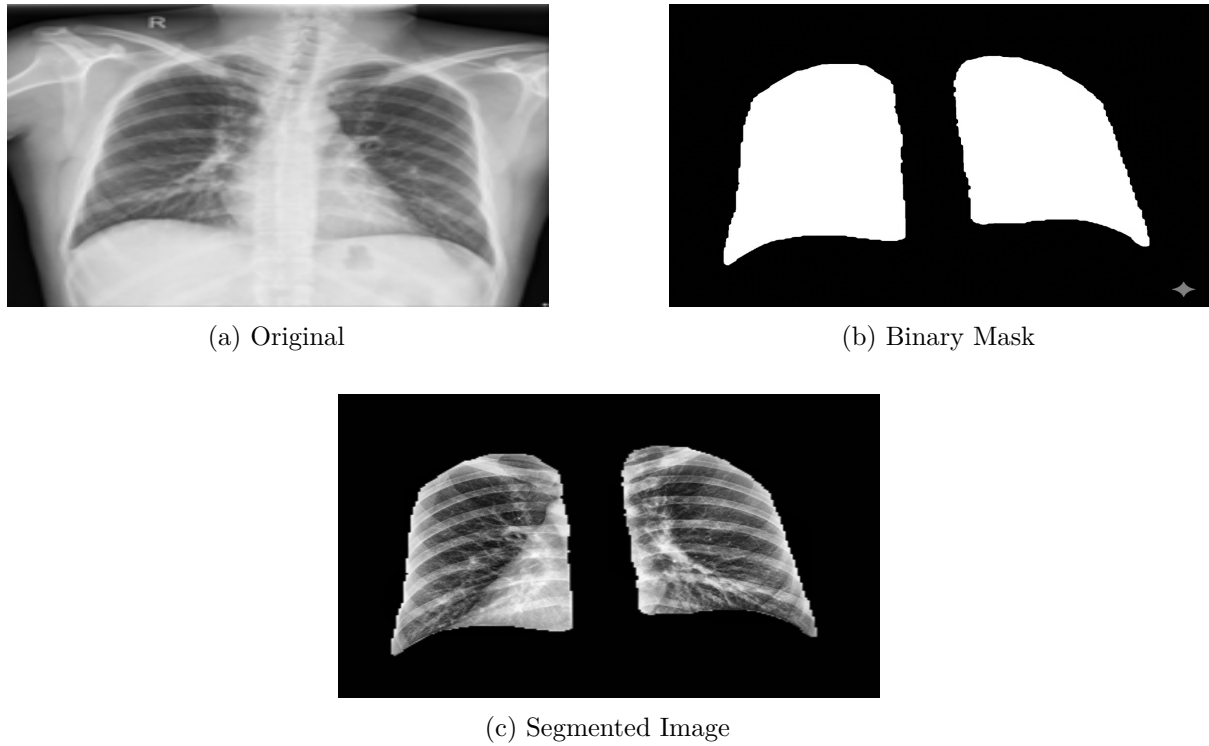
Figure 3.12: U-Net segmentation results. From left to right: the preprocessed input radiograph, the predicted binary lung mask, and the masked output image passed to the classification stage.
