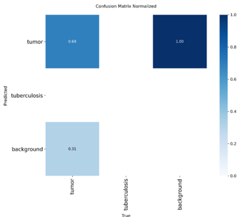
Figure 4.29: Normalized confusion matrix of the centralized YOLOv8n model.
