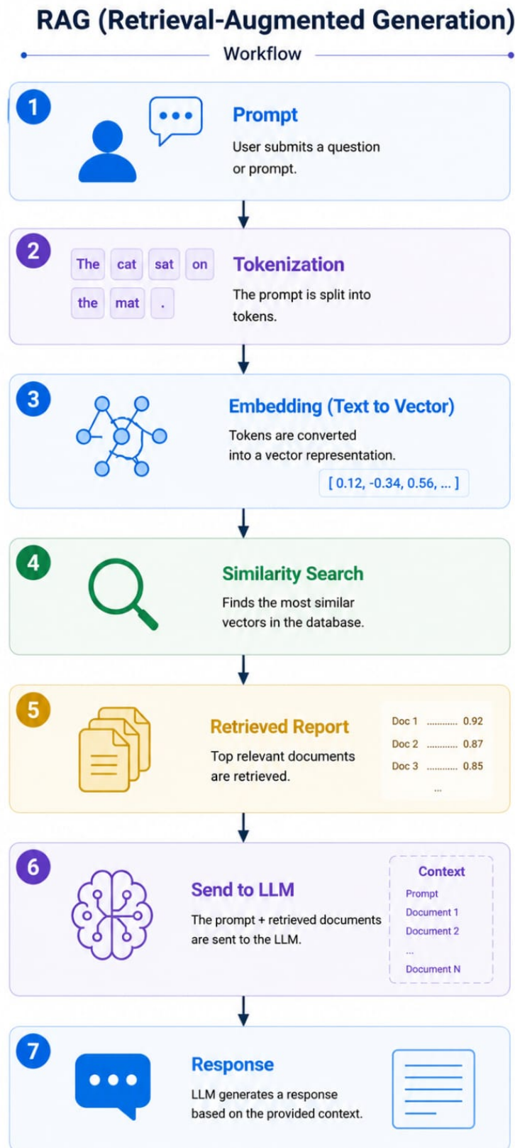
Figure 3.42: A simple visualization of the overall RAG architecture.
