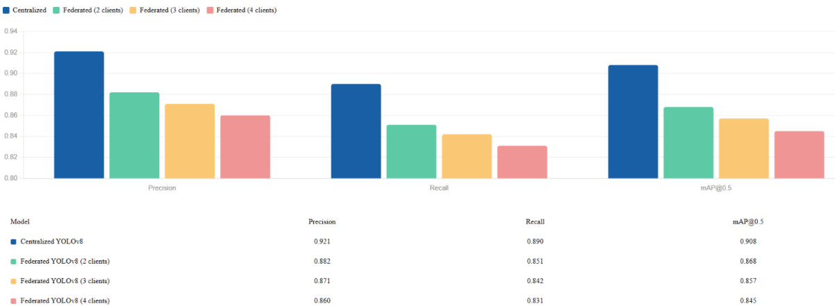
Figure 4.32: The full visualization of the results of the YOLOv8 architecture with tests on both centralized and federated frameworks with different clients in the case of the federated framework.
