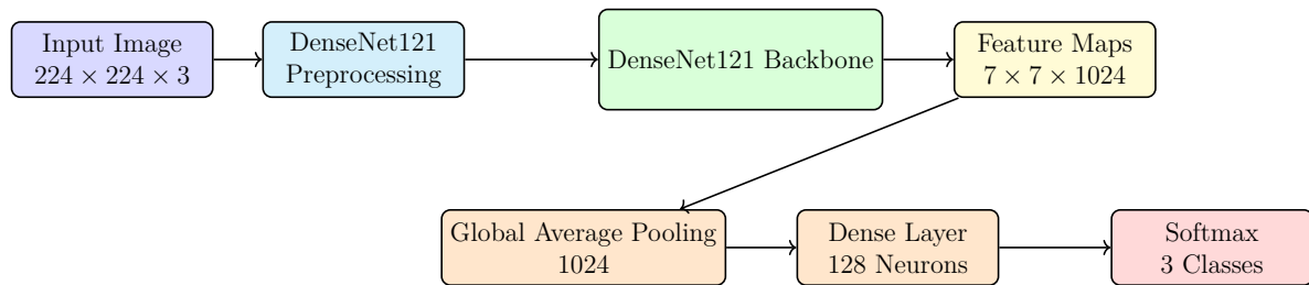
Figure 3.3: Two-row architecture of the DenseNet121-based medical image routing model.
