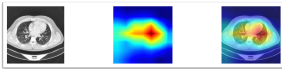
Figure 4.31: EfficientNet-B0 Grad-CAM visualization.
