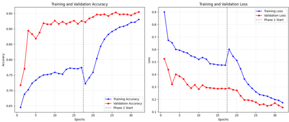
Figure 4.15: Learning curves for VGG-19 SoftMax.
