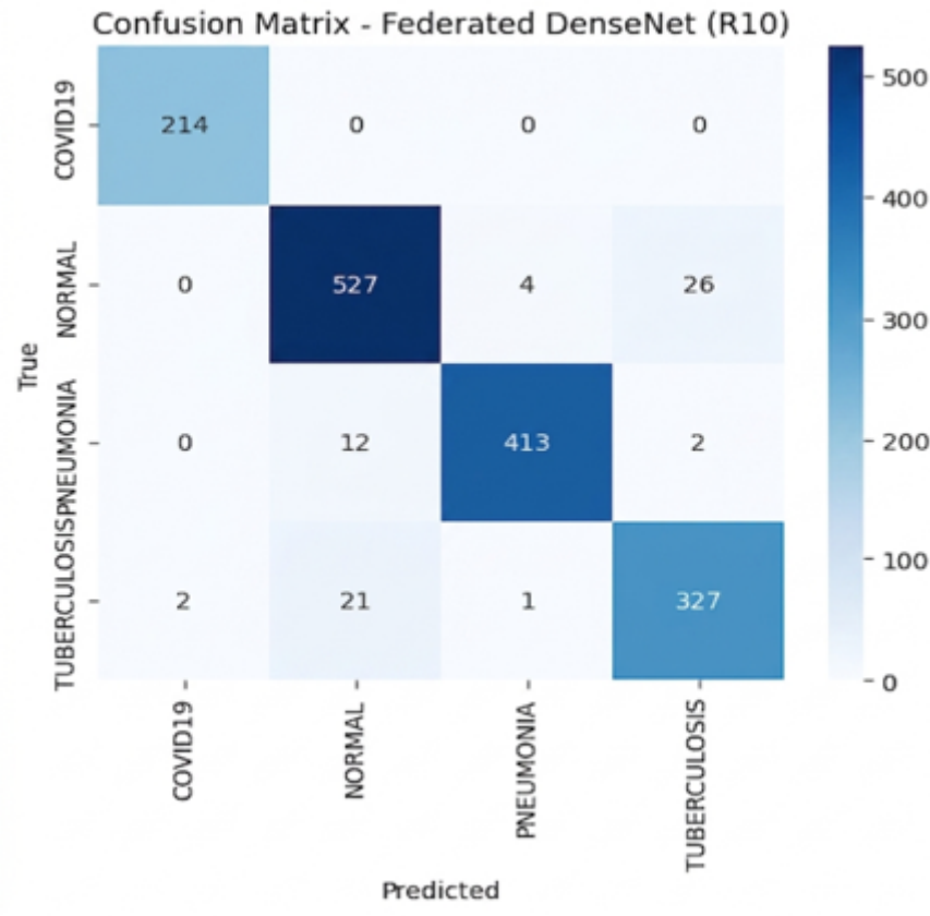
Figure 4.23: Confusion matrix for the Federated DenseNet121 model trained with 2 clients on the global held-out test set (accuracy: 95.57%).
