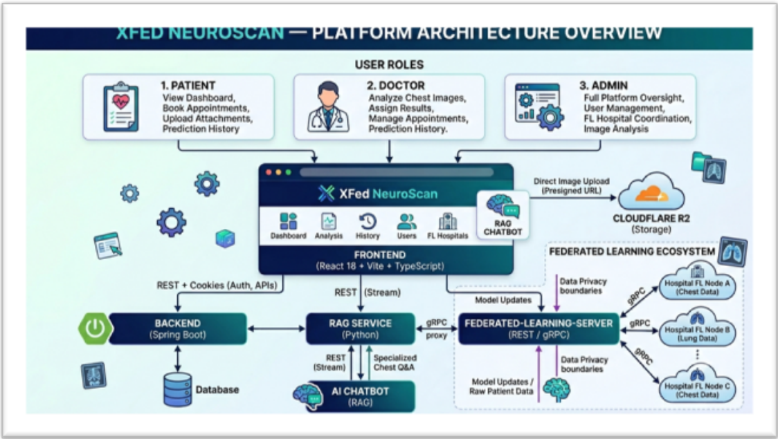
Figure 3.26: Deployment architecture of the proposed system showing the frontend application, backend services, model-serving infrastructure, federated learning server, databases, storage components, and external integrations.
