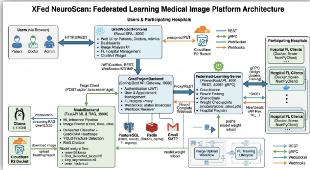
Figure 3.25: End-to-end logical architecture of the proposed X-Fed NeuroScan framework, illustrating the interaction between users, backend services, AI models, explainability components, federated learning infrastructure, and data storage systems.
