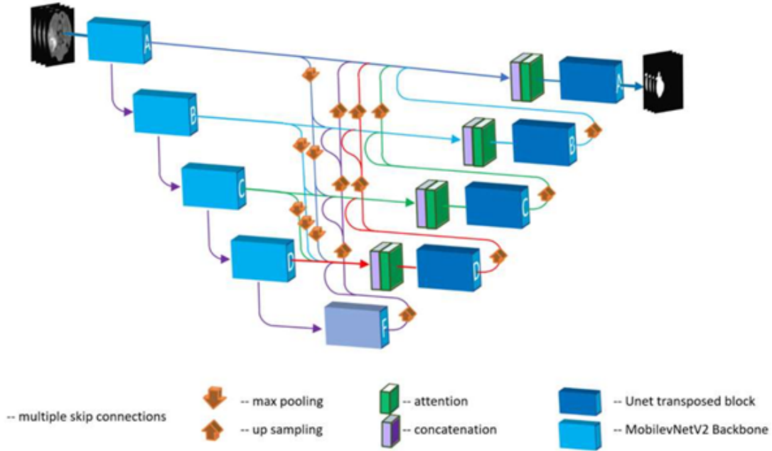
Figure 3.15: The U-Net architecture, illustrating the encoder-decoder structure with skip connections that merge high-resolution features from the contracting path with upsampled features in the expansive path. This design is highly effective for precise medical image segmentation.
