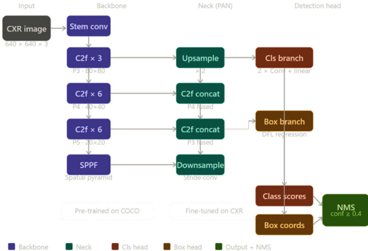
Figure 3.18: YOLOv8 architecture pipeline for automated localization and classification of pulmonary abnormalities.
