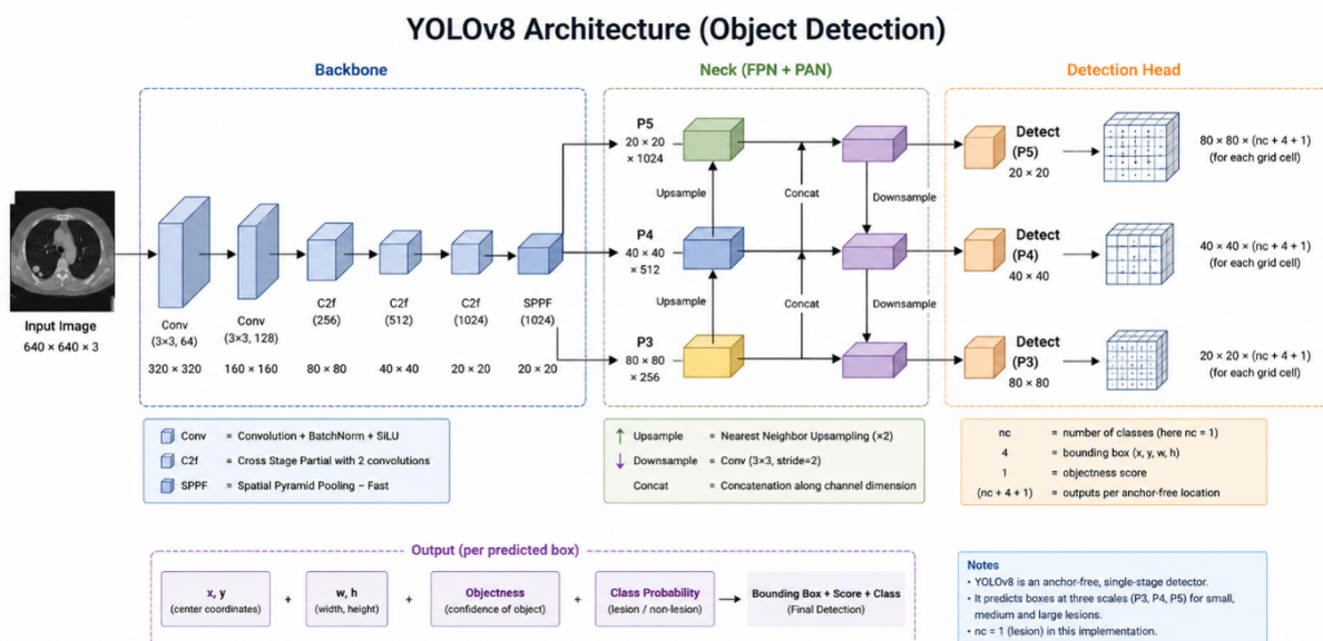
Figure 3.22: Detailed architectural diagram of the YOLOv8 object detection framework, illustrating the Backbone, Neck (FPN + PAN), and Detection Head stages for multi-scale prediction.
