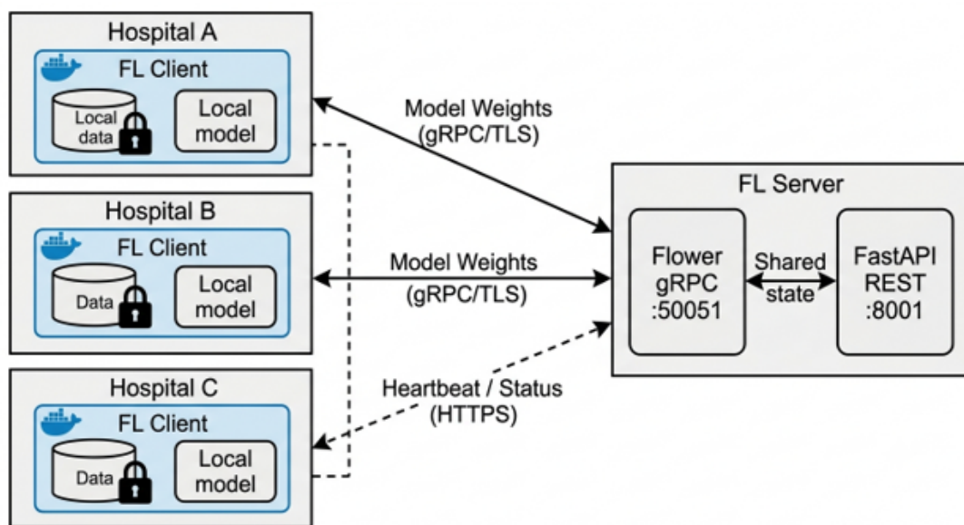
Figure 3.28: Two-tier federated learning system architecture. Hospital clients communicate with the central federated learning server through TLS-secured gRPC channels, while the REST management layer provides round lifecycle management and monitoring. Raw medical data remains within each hospital boundary.
