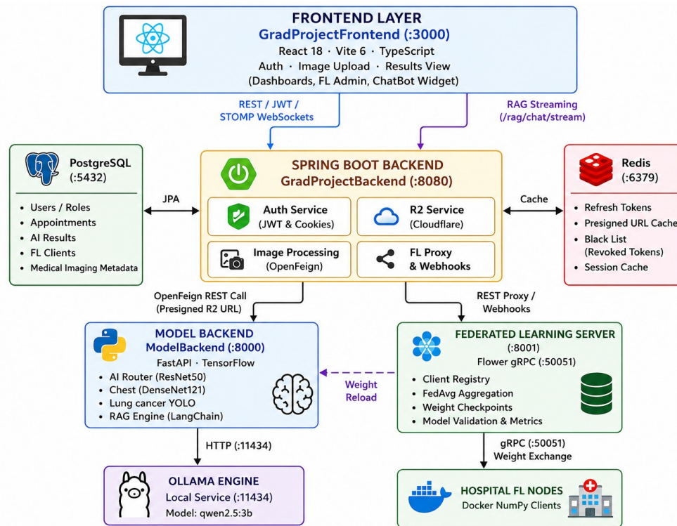
Figure 3.32: End-to-end logical architecture of the proposed X-Fed NeuroScan framework, illustrating the interaction between users, backend services, AI models, explainability components, federated learning infrastructure, and data storage systems.
