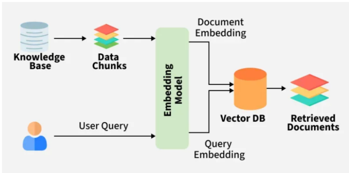
Figure 3.31: Query processing workflow of the proposed RAG system.
