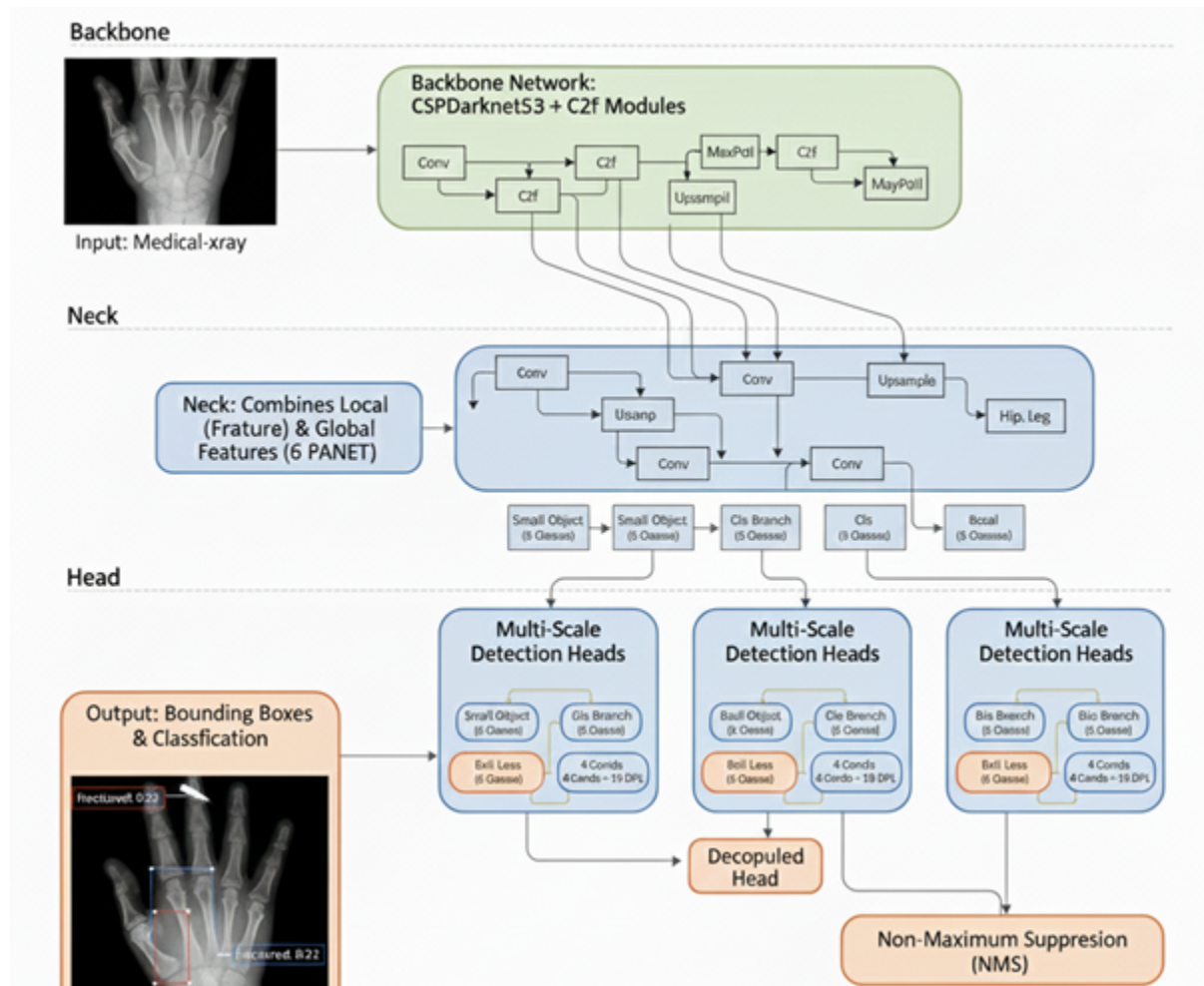
Figure 3.5: General architecture of YOLOv8 illustrating the backbone, neck, and detection head components.
