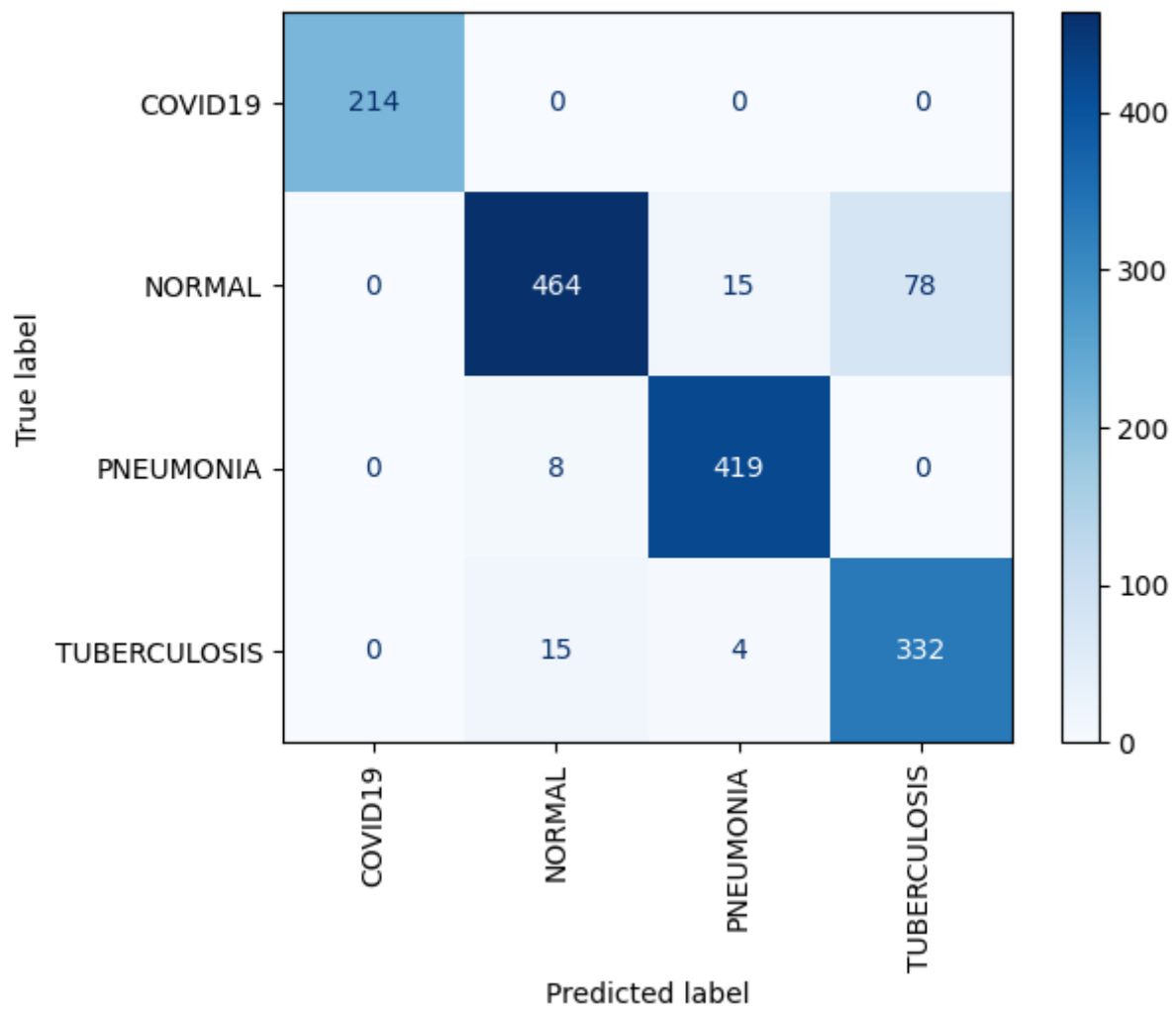
Figure 4.14: Confusion matrix for EfficientNet SoftMax.
