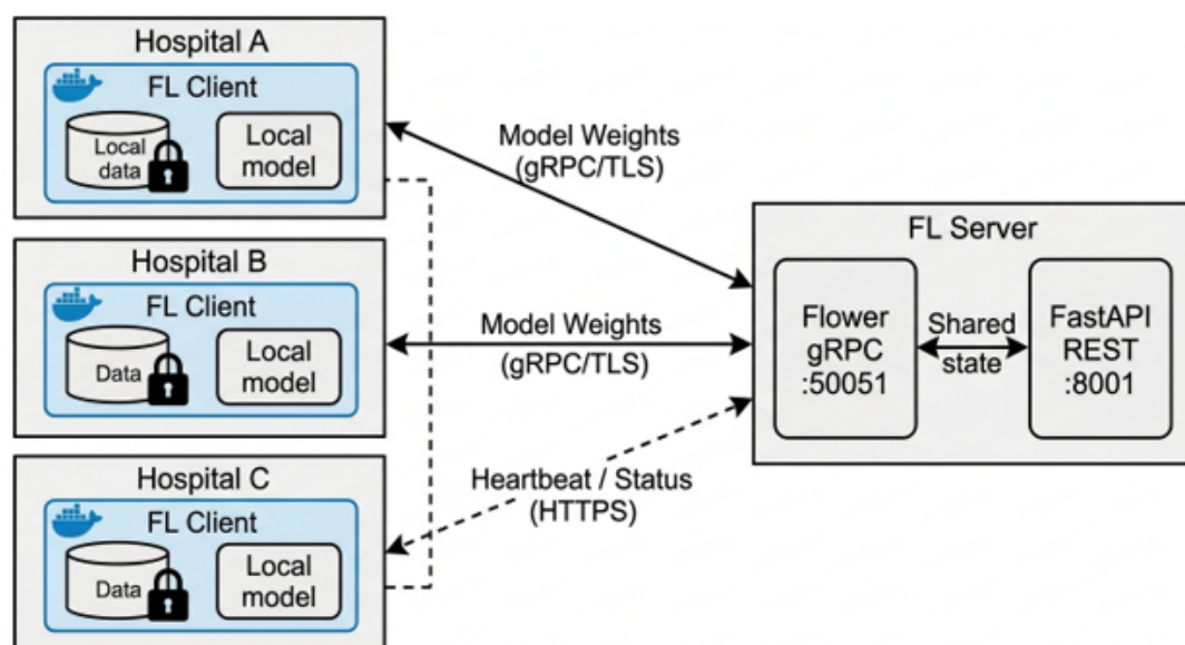
Figure 3.21: Two-tier federated learning system architecture. Hospital clients communicate with the central federated learning server through TLS-secured gRPC channels, while the REST management layer provides round lifecycle management and monitoring. Raw medical data remains within each hospital boundary.
