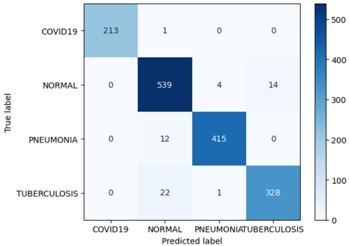
Figure 4.10: Confusion matrix for ResNet50V2 SoftMax.
