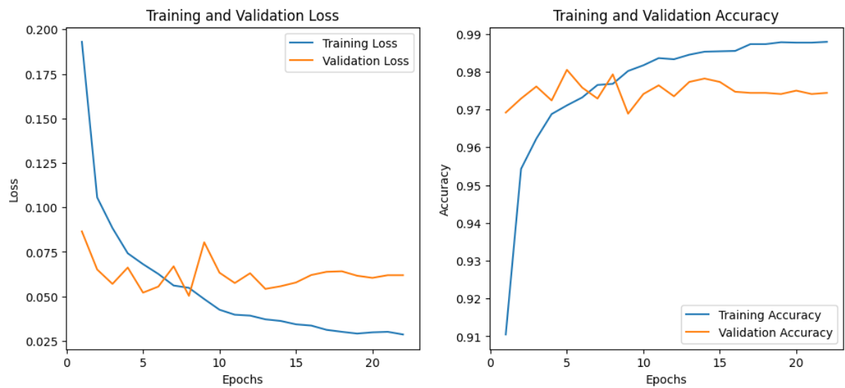
Figure 4.20: Learning curves for DenseNet121 OVR.
