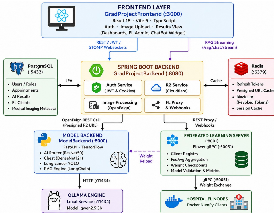
Figure 3.25: End-to-end logical architecture of the proposed X-Fed NeuroScan framework, illustrating the interaction between users, backend services, AI models, explainability components, federated learning infrastructure, and data storage systems.
