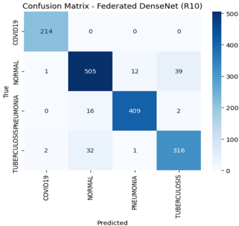
Figure 4.27: Confusion matrix for the Federated DenseNet121 model trained with 4 clients (accuracy: 93.22%).
