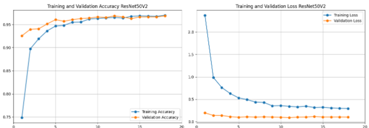
Figure 4.9: Learning curves for ResNet50V2 SoftMax.
