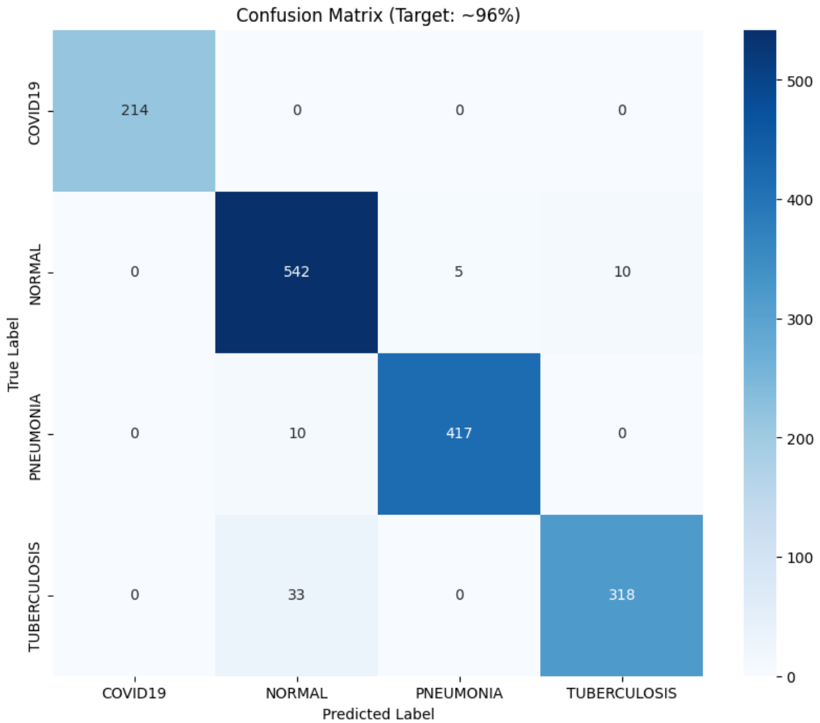
Figure 4.19: Confusion matrix for ResNet50 OVR.
