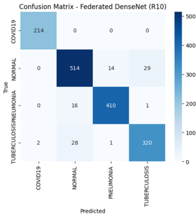
Figure 4.25: Confusion matrix for the Federated DenseNet121 model trained with 3 clients.
