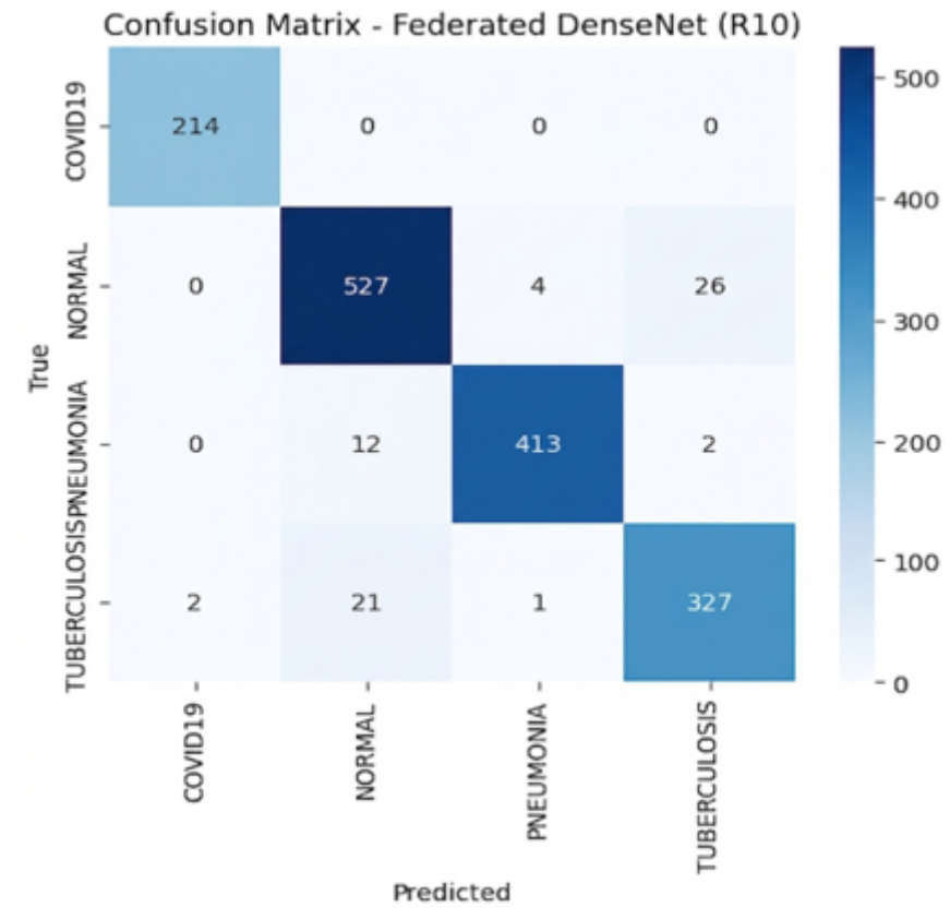
Figure 4.23: Confusion matrix for the Federated DenseNet121 model trained with 2 clients on the global held-out test set (accuracy: 95.57%).
