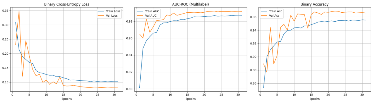
Figure 4.18: Learning curves for ResNet50 OVR.
