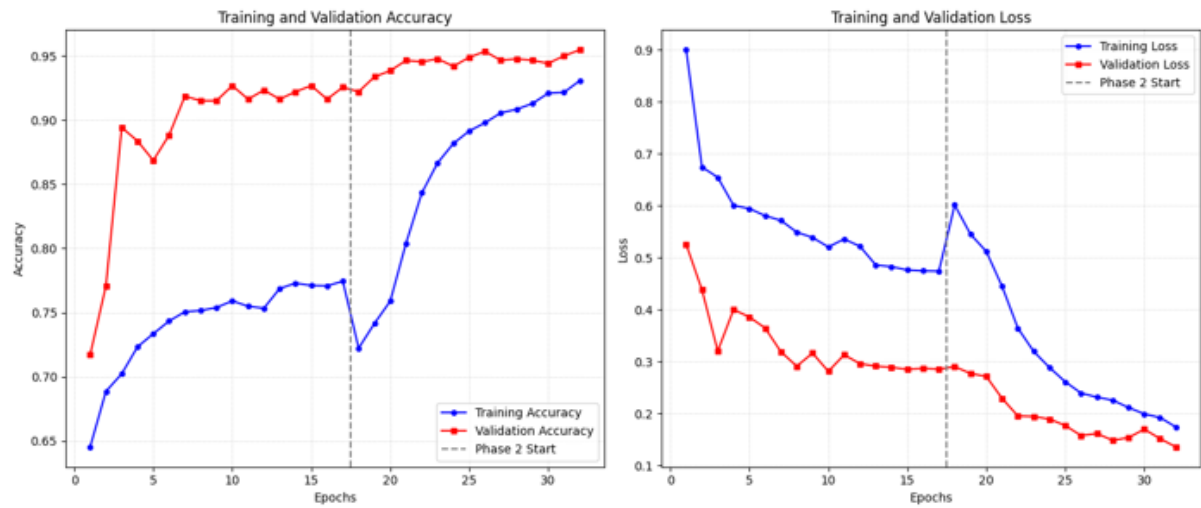
Figure 4.15: Learning curves for VGG-19 SoftMax.
