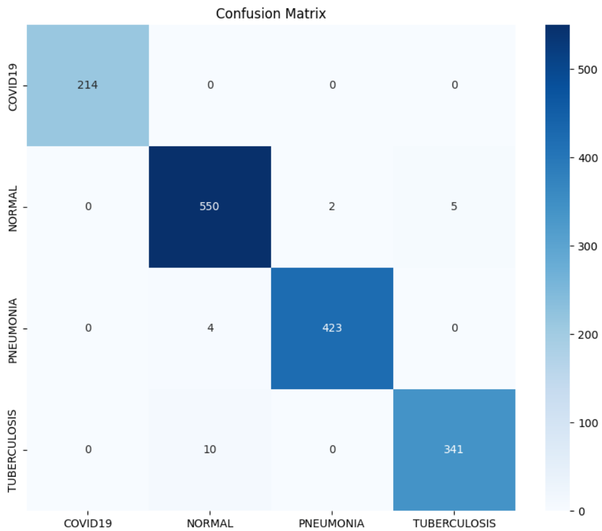
Figure 4.21: Confusion matrix for DenseNet121 OVR.
