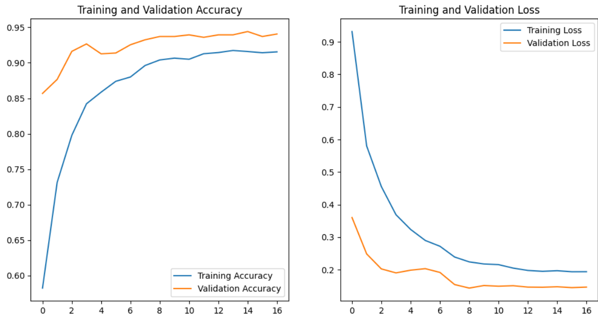
Figure 4.13: Learning Curves for EfficientNet SoftMax.
