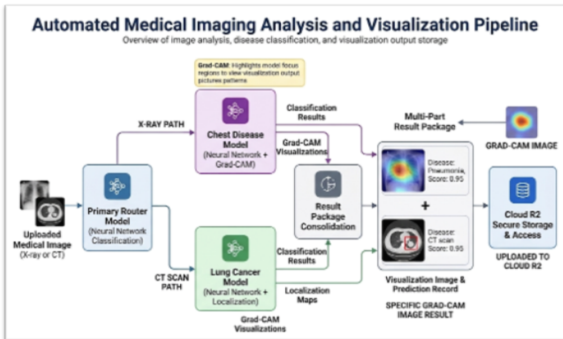
Figure 3.41: A simple visualization of the overall image processing pipeline from the backend's perspective.
