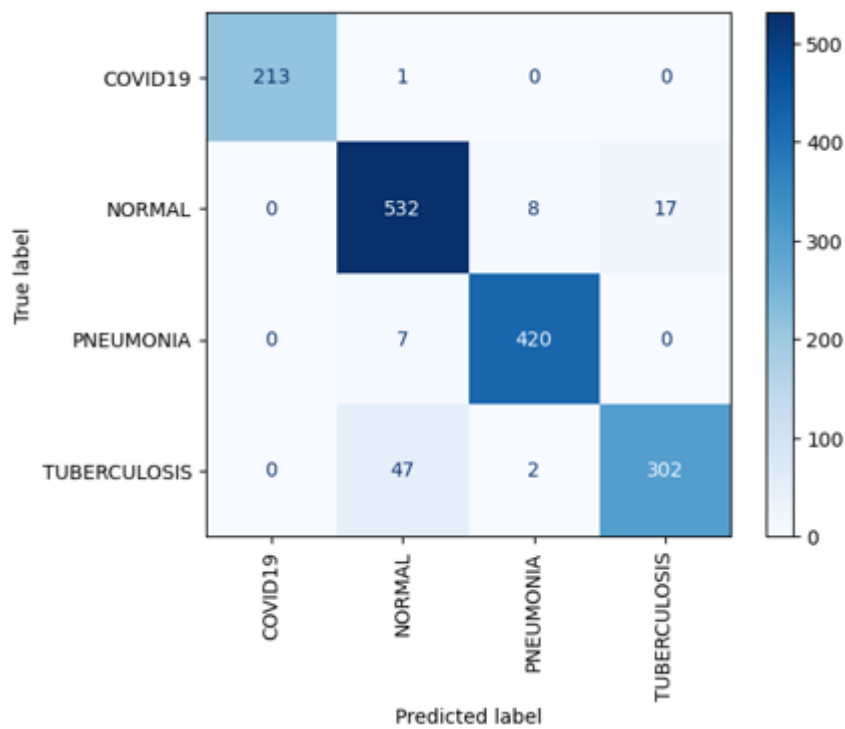
Figure 4.16: Confusion matrix for VGG-19 SoftMax.
